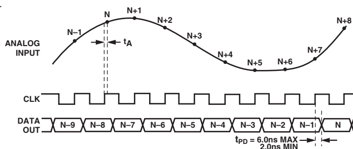
Figure 1. Timing Diagram
