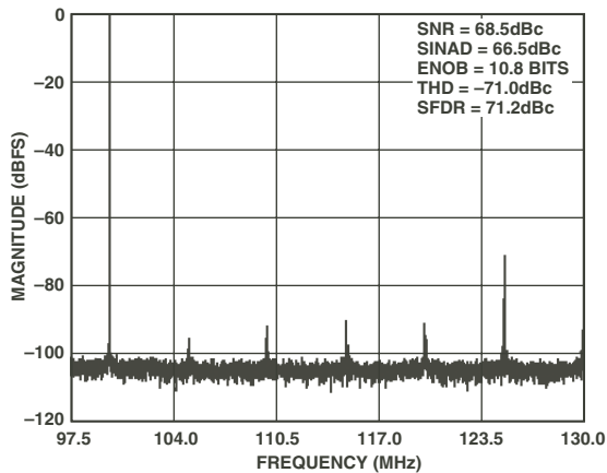
TPC 3. Single Tone 8K FFT with f_{\text{IN}} = 100 \text{ MHz}
