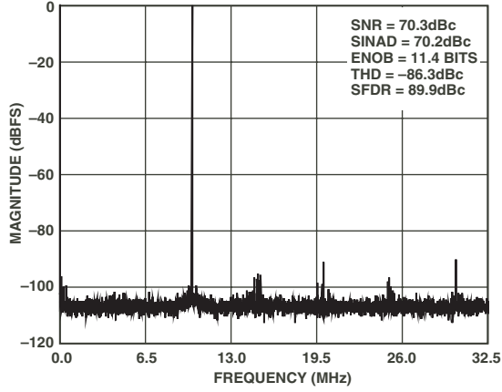
TPC 1. Single Tone 8K FFT with f_{\text{IN}} = 10 \text{ MHz}
