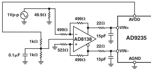
Figure 8. Differential Input Configuration Using the AD8138
