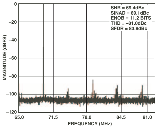
TPC 2. Single Tone 8K FFT with f_{\text{IN}} = 70 \text{ MHz}
