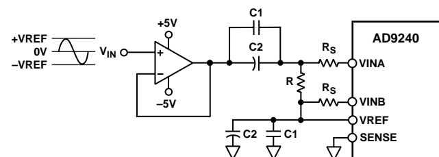
Figure 37. AC-Coupled Input
