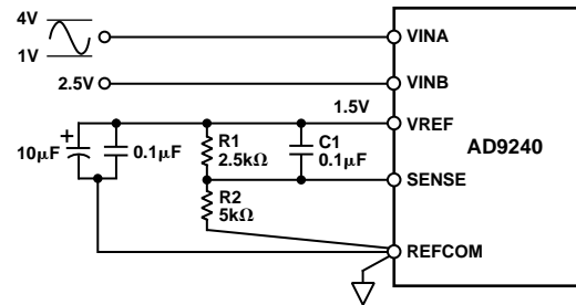
Figure 41. Resistor Programmable Reference (3 V p-p Input Span, V_{CM} = 2.5 V)
