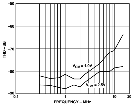
Figure 27. THD vs. Frequency for V_{CM} = 2.5\text{ V} and 1.0\text{ V} ( A_{IN} = -0.5\text{ dB} , Input Span = 2.0\text{ V p-p} )
