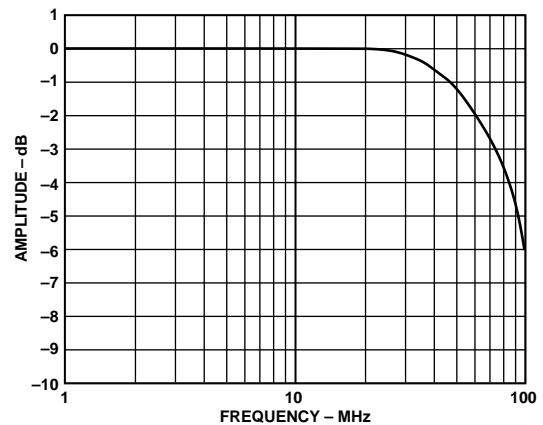
Figure 25. Full-Power Bandwidth
