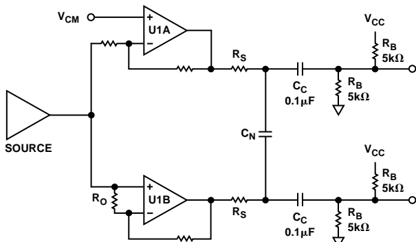
Figure 33. AC Coupling of Op Amps
