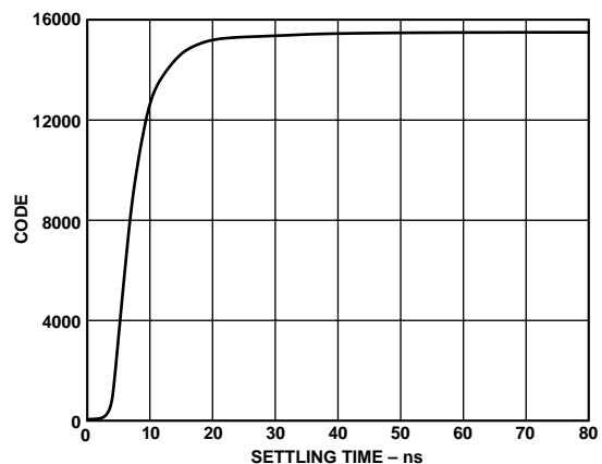
Figure 26. Settling Time
