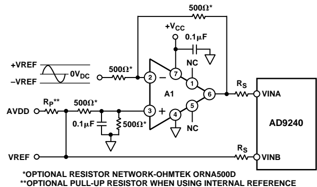
Figure 36. Single-Ended Input With DC-Coupled Level-Shift
