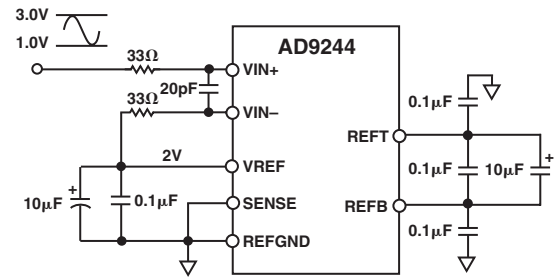
Figure 3b. 2 V p-p Single-Ended Input, Common-Mode Voltage = 2 V
