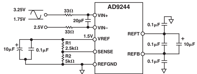
Figure 10. Resistor Programmable Reference (1.5 V p-p Input Span, Differential Input with VCM = 2.5 V)
