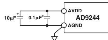
Figure 17. Analog Supply Decoupling
