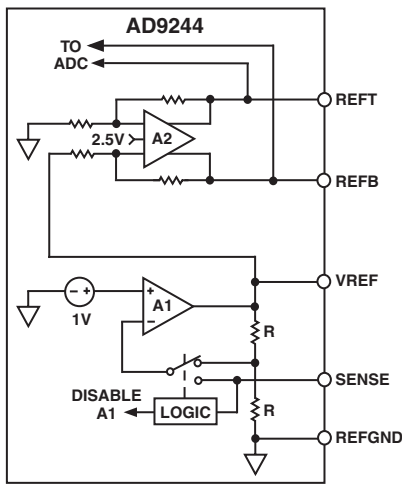
Figure 9a. Equivalent Reference Circuit
