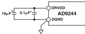
Figure 18. Digital Supply Decoupling
