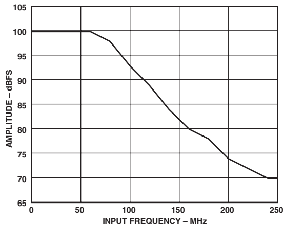
TPC 27. CMRR vs. Input Frequency ( A_{IN} = 0 dBFS and CML = 2.5 V)
