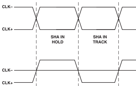
Figure 14. SHA Timing
