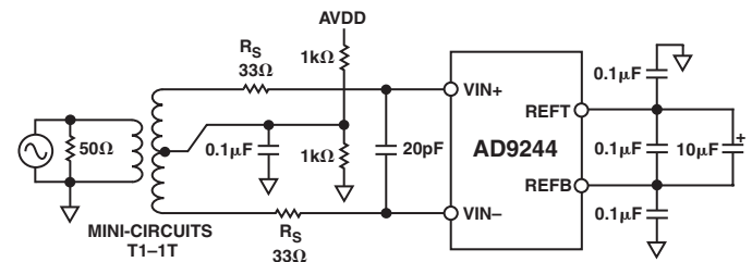
Figure 7. Transformer-Coupled Input
