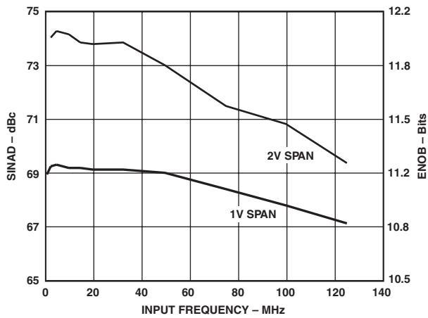
TPC 7. SINAD/ENOB vs. Input Frequency
