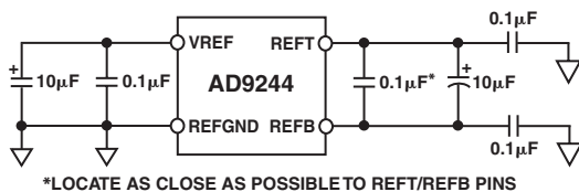
Figure 9b. Reference Decoupling
