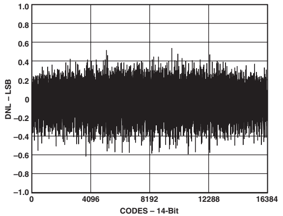
TPC 18. Typical DNL
