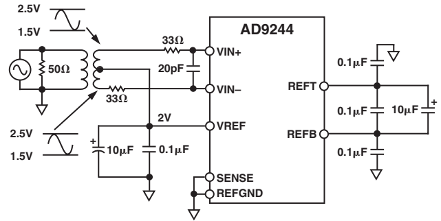
Figure 3a. 2 V p-p Differential Input, Common-Mode Voltage = 2 V
