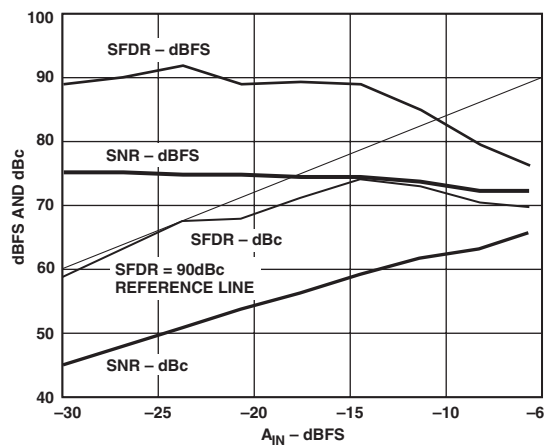
TPC 24. Dual-Tone SNR/SFDR vs. A_{IN} with f_{IN-1} = 139.2 MHz and f_{IN-2} = 140.7 MHz
