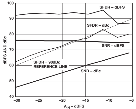
TPC 22. Dual-Tone SNR/SFDR vs. A_{IN} with f_{IN-1} = 44.2 MHz and f_{IN-2} = 45.6 MHz
