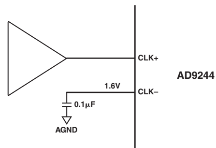
Figure 15b. Single-Ended Clock Input—DC-Coupled
