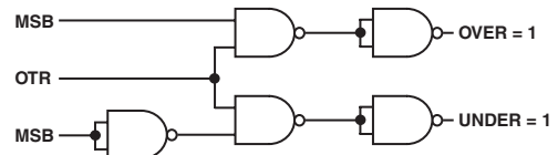
Figure 13. Overage/Underrange Logic
