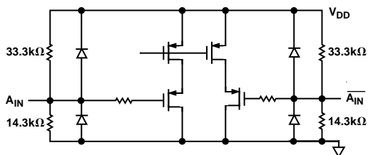
Figure 2. Equivalent Analog Input Circuit
