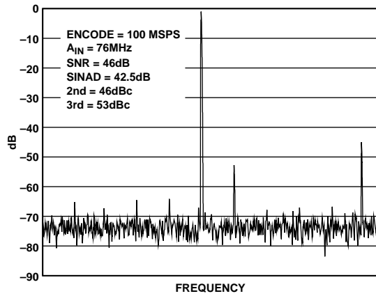
Figure 9. Spectrum: f_s = 100\text{ MSPS} , f_{IN} = 76\text{ MHz}
