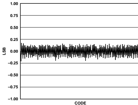
Figure 18. Differential Nonlinearity
