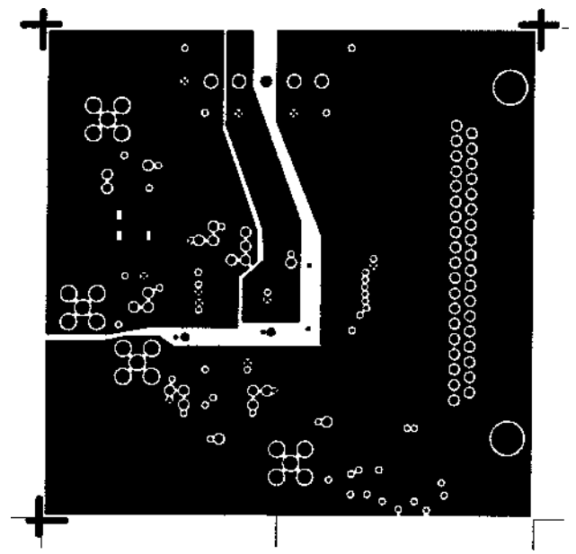
Figure 23. Printed Circuit Board "Split" Power Layer
