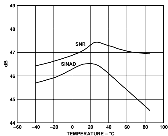
Figure 17. SINAD/SNR vs. Temperature
