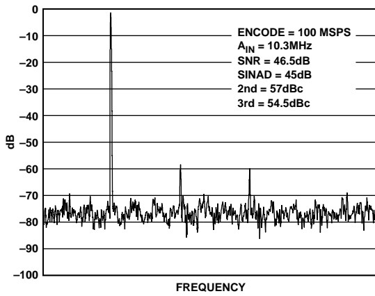
Figure 7. Spectrum: f_s = 100\text{ MSPS} , f_{IN} = 10.3\text{ MHz}
