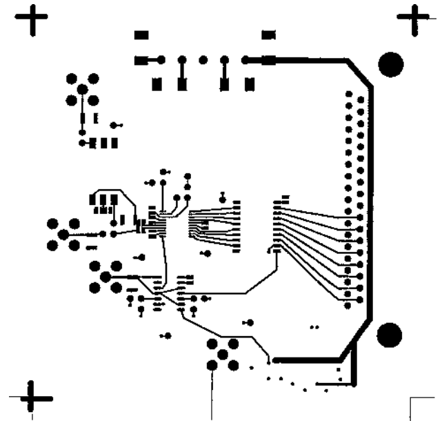
Figure 22. Printed Circuit Board Top Side Copper
