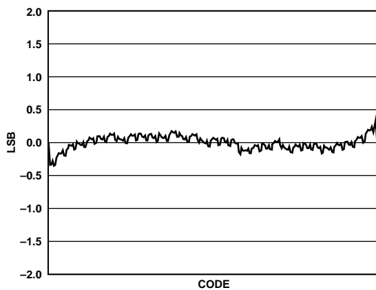
Figure 19. Integral Nonlinearity
