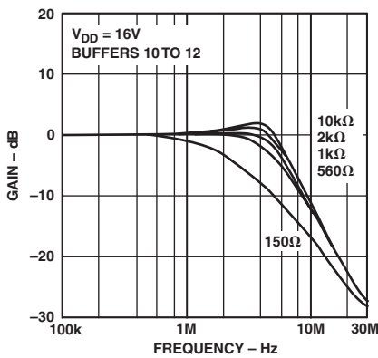
TPC 16. Frequency Response vs. Resistive Loading
