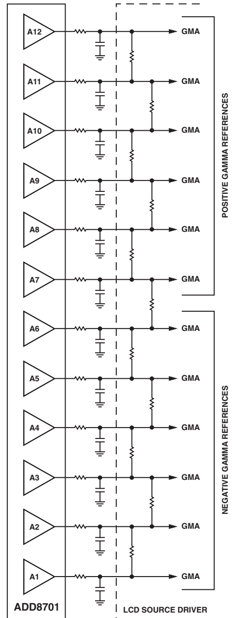
Figure 2. Application Circuit
