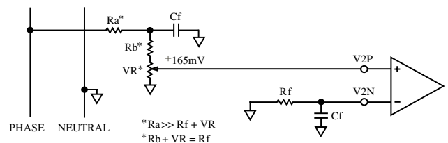
Figure 16. Typical Connections for Channel V2
