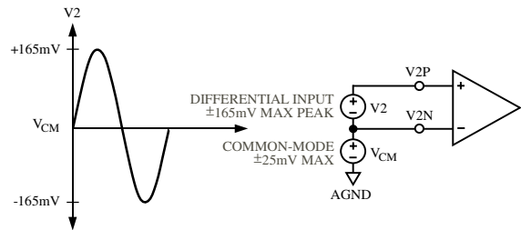
Figure 14. Maximum Signal Levels, Channel V2
