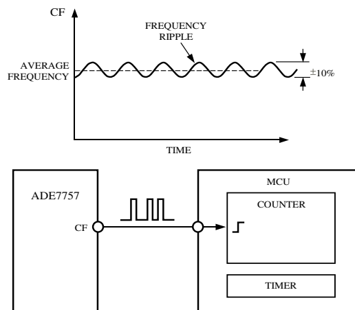
Figure 22. Interfacing the ADE7757 to an MCU
