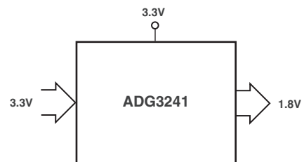
Figure 9. 3.3 V to 1.8 V Voltage Translation, \overline{SEL} = 0\text{ V}
