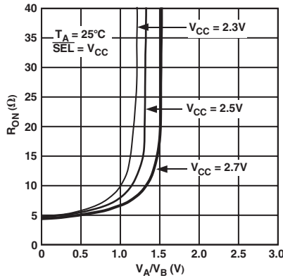
TPC 2. On Resistance vs. Input Voltage
