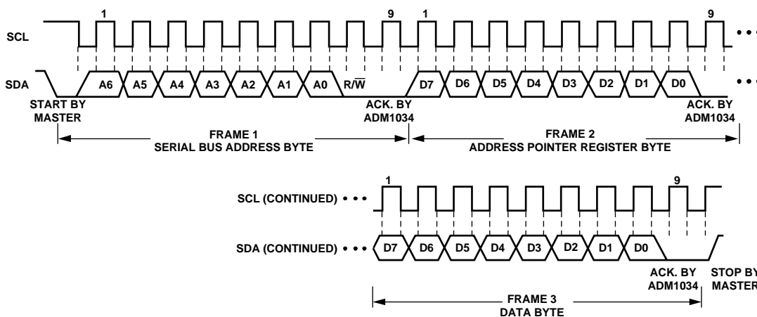
Figure 18. Writing a Register Address to the Address Pointer Register, then Writing Data to the Selected Register
