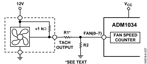
Figure 39. Fan with Strong TACH. Pull-Up to >V_{CC} or Totem-Pole Output, Attenuated with R_1/R_2 .
