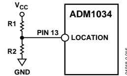
Figure 16. Bootstrapping the LOCATION Input
