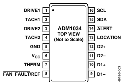
Figure 3. Pin Configuration
