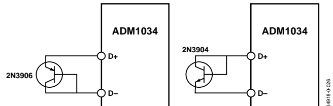
Figure 27. Measuring Temperature by Using Discreet Transistors
