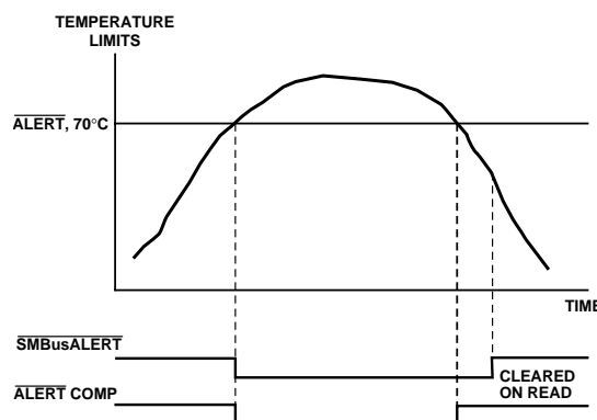
Figure 31. ALERT Comparator and SMBusALERT Outputs
