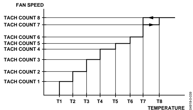
Figure 41. Programming the Look-Up Table in Discreet Fan Speeds Mode
