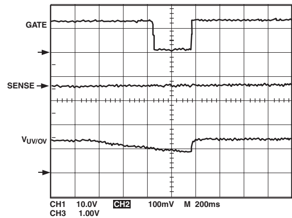
Figure 8. Timing Waveforms Associated with an Undervoltage Glitch
