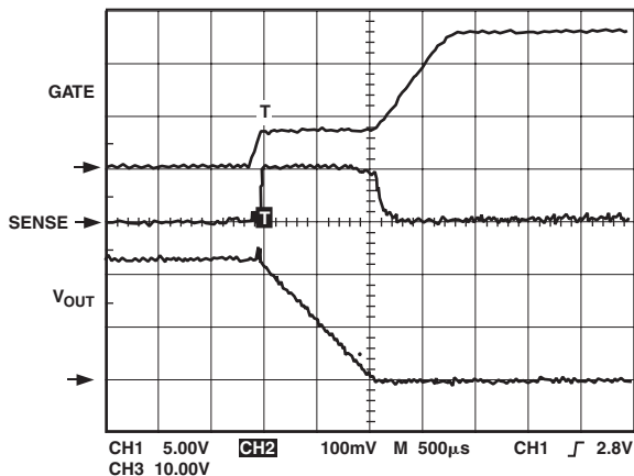
Figure 6. Start-Up Sequence
