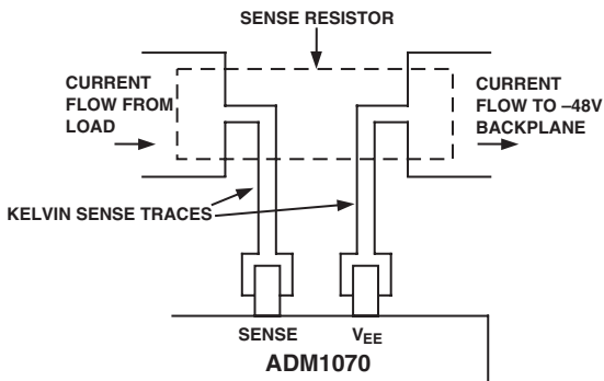
Figure 14. Kelvin Sensing with the ADM1070
