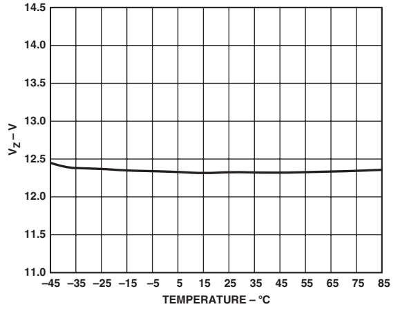
TPC 4. V_Z vs. Temperature
