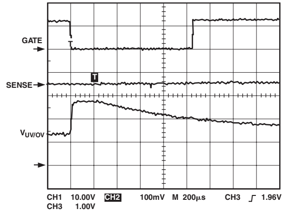
Figure 7. Timing Waveforms Associated with an Overvoltage Glitch
