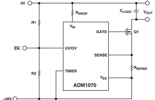
Figure 15. UV/OV Used as Enable Input
