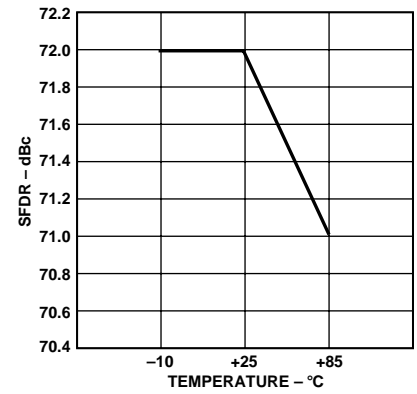
Figure 4. SFDR vs. Temperature @ f_{CLK} = 50\text{ MHz} ( f_{OUT} = 1\text{ MHz} )
