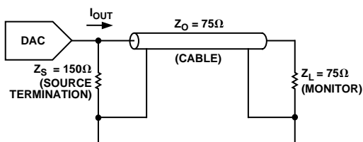
Figure 23. Analog Output Termination for RS-170
