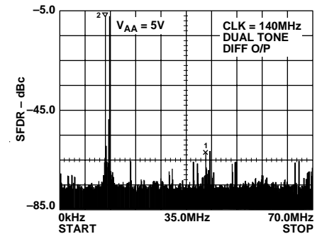
Figure 10. Dual-Tone SFDR @ f_{CLK} = 140\text{ MHz} ( f_{OUT1} = 13.5\text{ MHz} , f_{OUT2} = 14.5\text{ MHz} )
