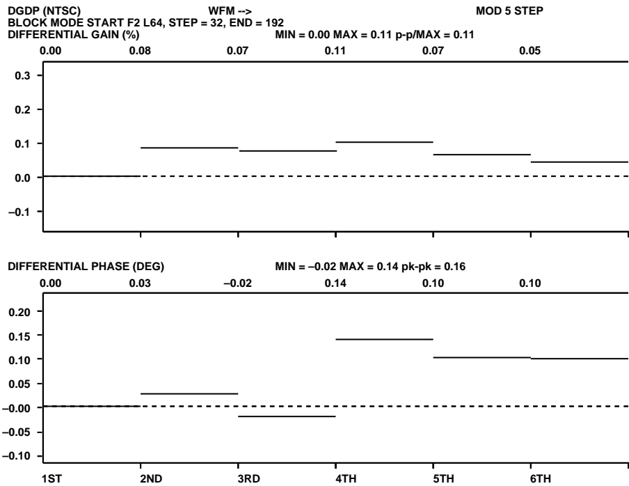
Figure 94. NTSC Differential Gain and Phase Measurement
