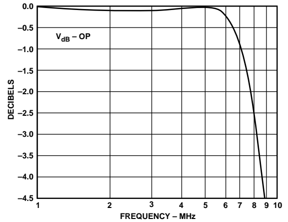
Filter 82. Output Filter Plot Close-Up
