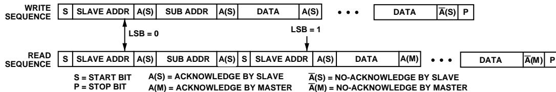
Figure 36. Write and Read Sequences
