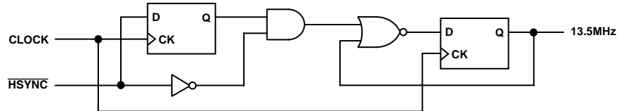
Figure 55. Circuit to Generate 13.5 MHz
