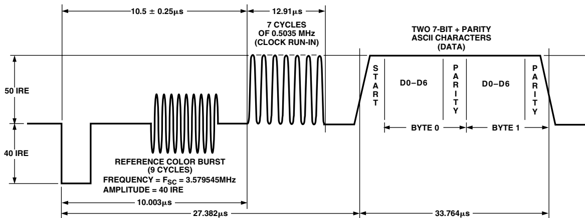
Figure 96. Closed Captioning Waveform (NTSC)
