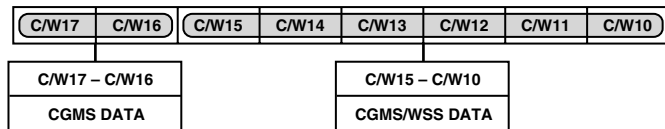
Figure 77. CGMS_WSS Register 1
