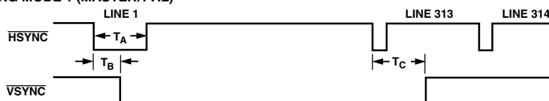
Figure 68. Timing Register 1
