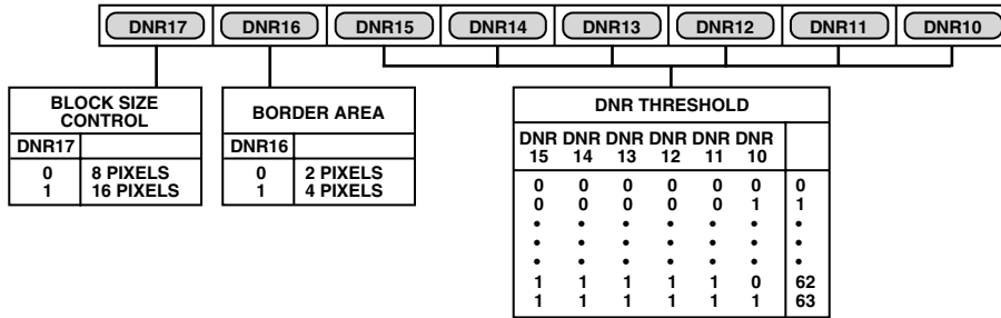
Figure 87. DNR Register 1
