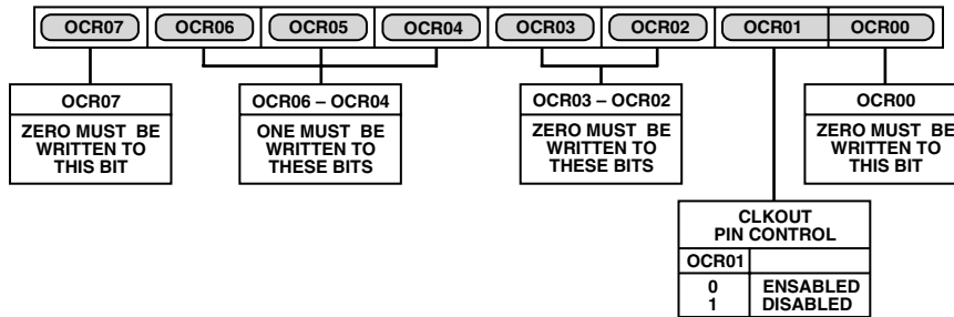
Figure 94. Output Clock Register
