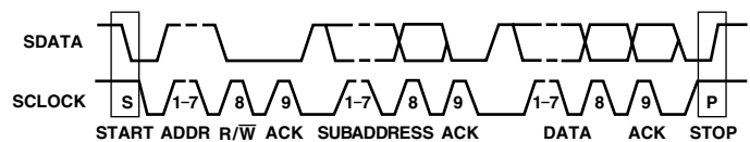
Figure 53. Bus Data Transfer
