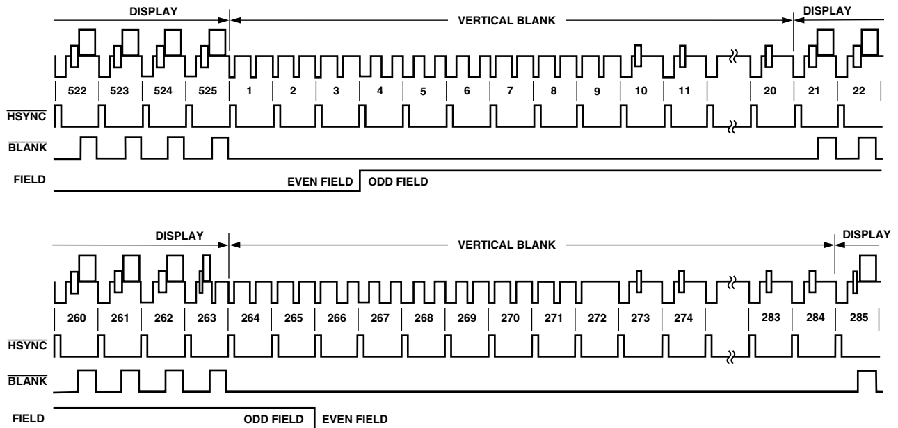
Figure 50. Timing Mode 3, NTSC
