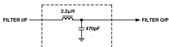
Figure 103. Output Filter for 4× Oversampling Mode
