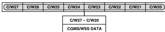
Figure 78. CGMS_WSS Register 2
