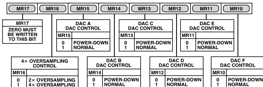
Figure 57. Mode Register 1, MR1
