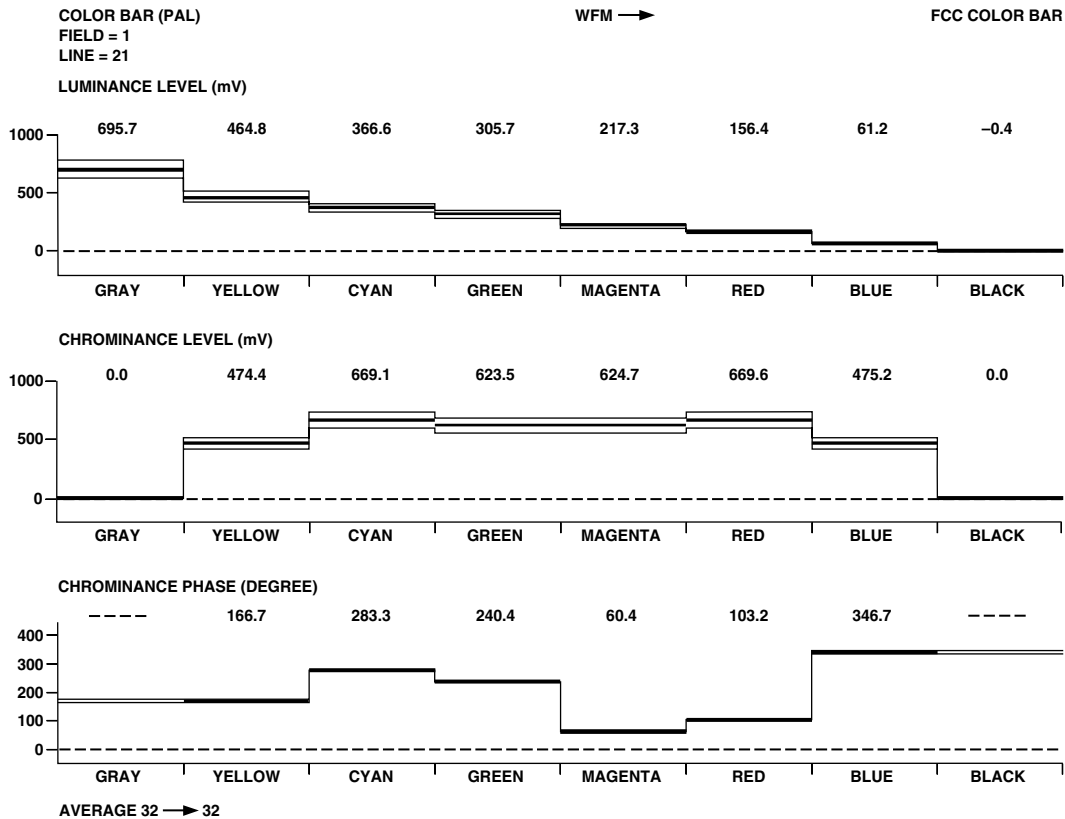
Figure 121. PAL Color Bar Measurement
