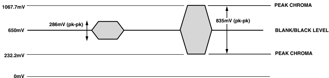
Figure 110. NTSC Chroma Video Levels
