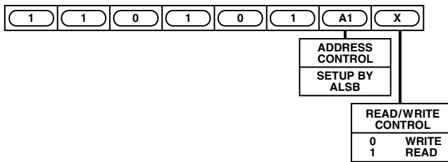
Figure 52. Slave Address
