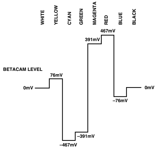
Figure 138. NTSC 100% Color Bars with Pedestal V
