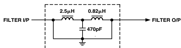
Figure 101. Output Filter for 2× Oversampling Mode
