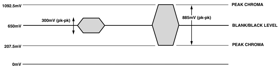
Figure 118. PAL Chroma Video Levels
