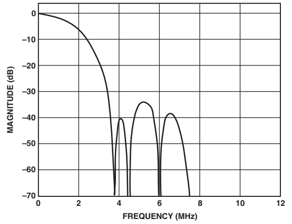
TPC 22. Chroma 1.3 MHz LP Filter
