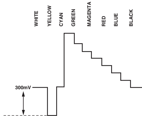
Figure 104. Y Levels—PAL
