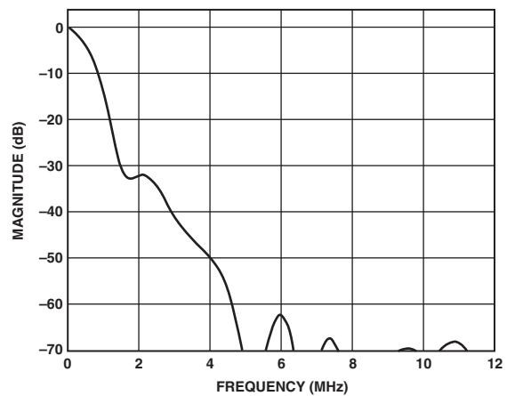
TPC 24. Chroma QCIF LP Filter
