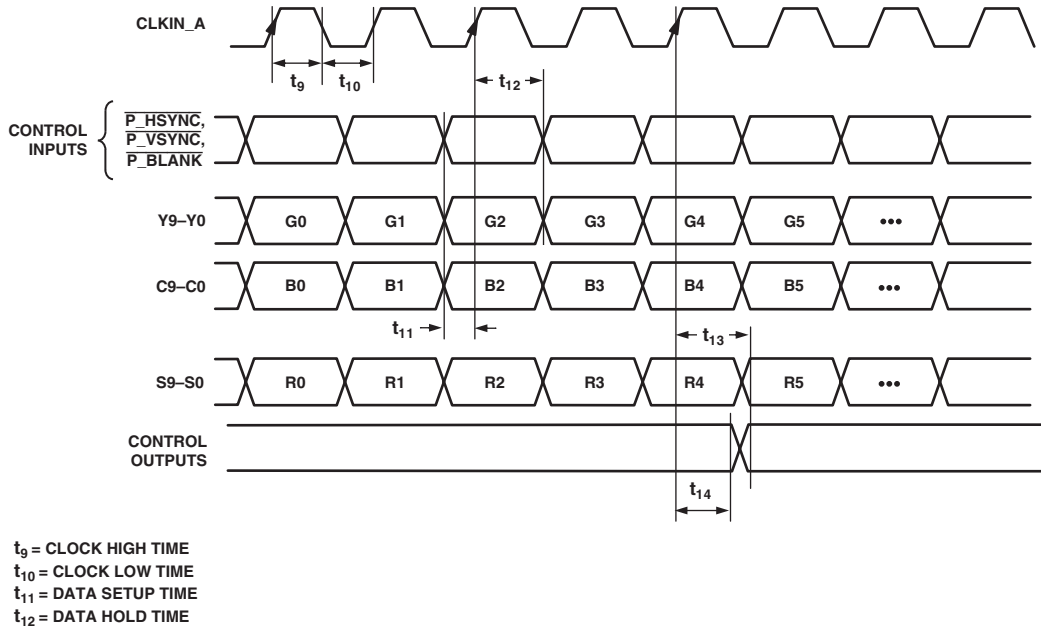
Figure 3. HD RGB 4:4:4 Input Mode [Input Mode 010]
