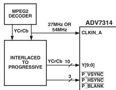
Figure 27. 1x 10-Bit PS at 27 MHz or 54 MHz
