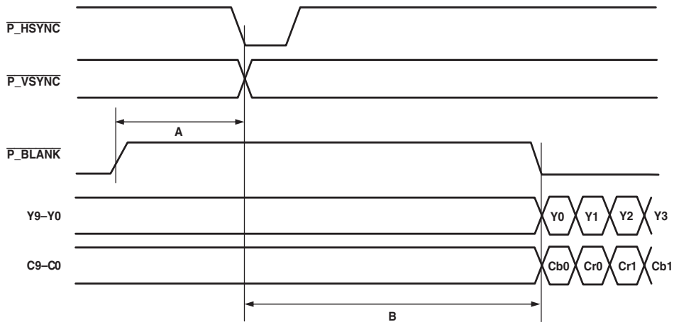
Figure 12. 20-/16-Bit SD Only Pixel Input Mode [Input Mode 000]
