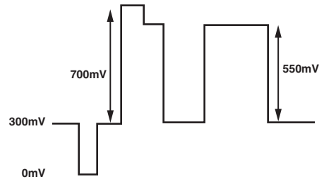
Figure 98. SD RGB Output Levels—RGB Sync Enabled
