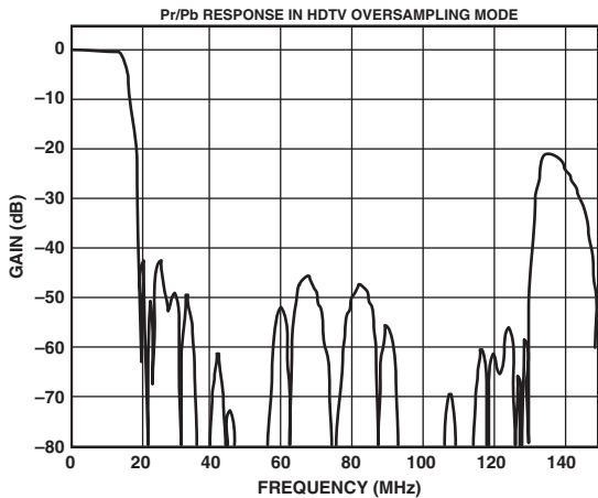
TPC 3. HDTV - UV 2x Oversampling Filter
