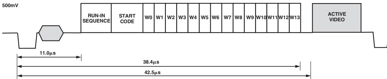
Figure 65. WSS Waveform Diagram
