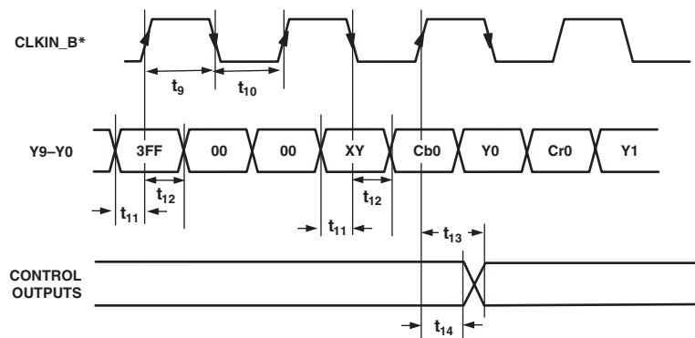
Figure 5. PS 4:2:2 1x10-Bit Interleaved at 54 MHz \overline{\text{HSYNC}}/\overline{\text{VSYNC}} Input Mode [Input Mode 111]
