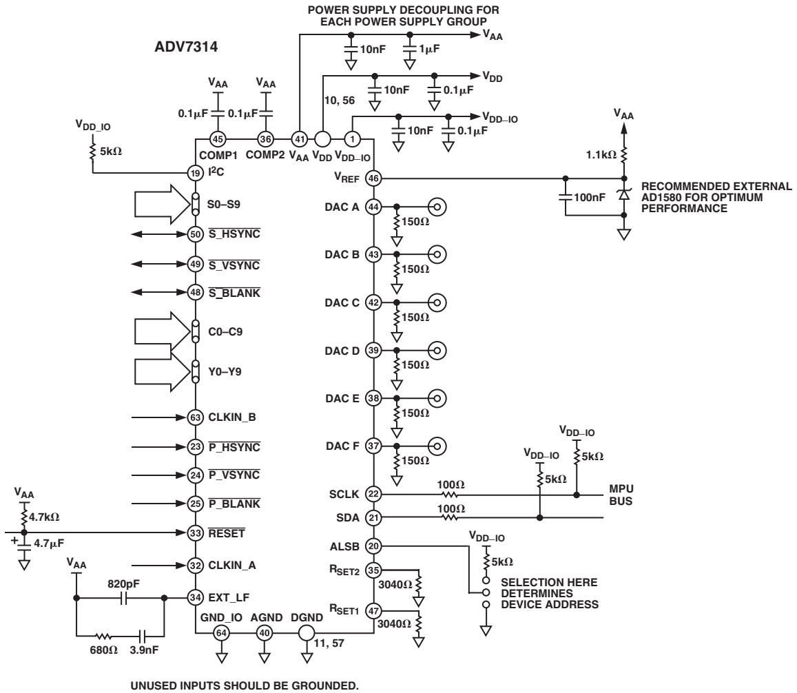
Figure 60. ADV7314 Circuit Layout
