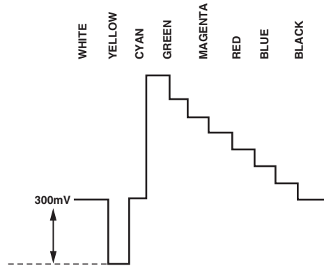
Figure 103. Y Levels—NTSC
