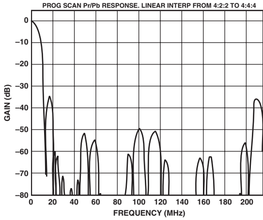
TPC 1. PS - UV 8x Oversampling Filter—Linear
