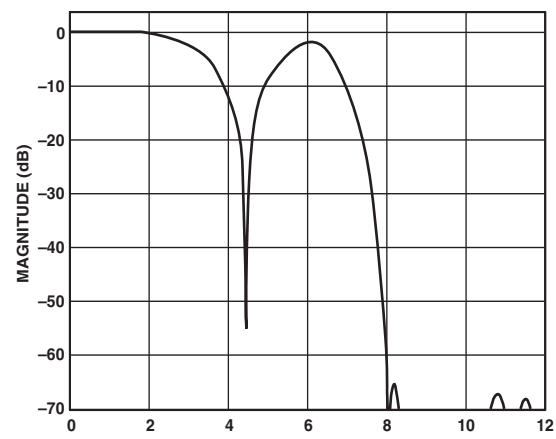
TPC 11. Luma PAL Notch Filter
