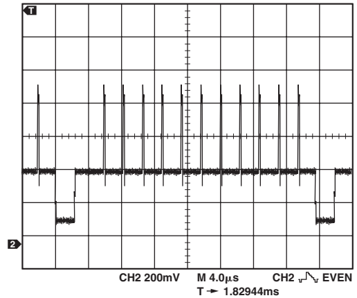
Figure 71. 525p Hatch Pattern
