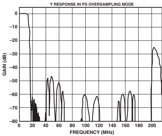
TPC 2. PS - Y 8x Oversampling Filter
