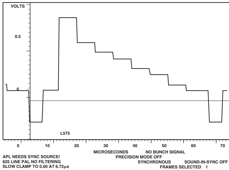
Figure 110. PAL Luma
