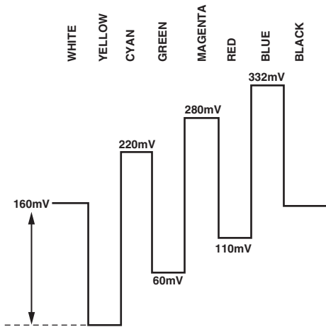
Figure 100. U Levels—PAL
