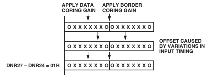
Figure 48. DNR Block Offset Control
