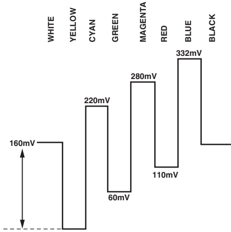
Figure 99. U Levels—NTSC
