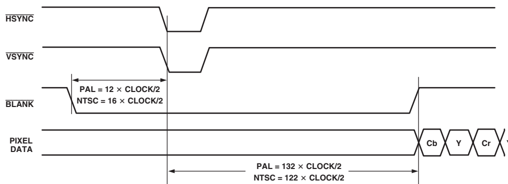
Figure 86. SD Timing Mode 2 Even-to-Odd Field Transition Master/Slave
