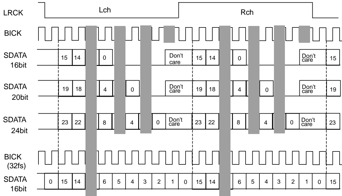
Figure 12. Mode 3 Timing
