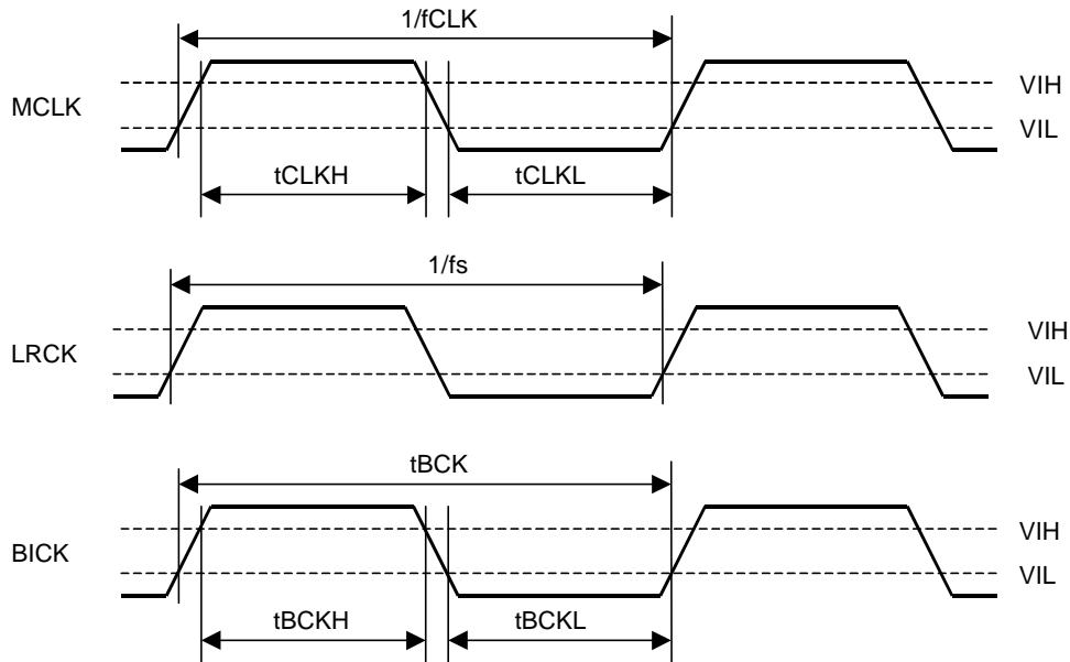
Figure 4. Clock Timing
