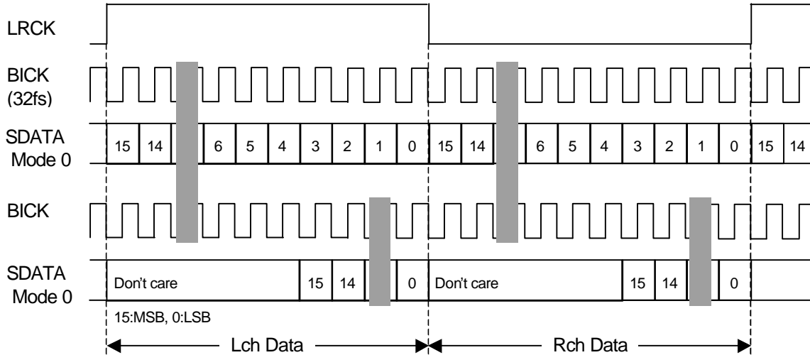
Figure 9. Mode 0 Timing
