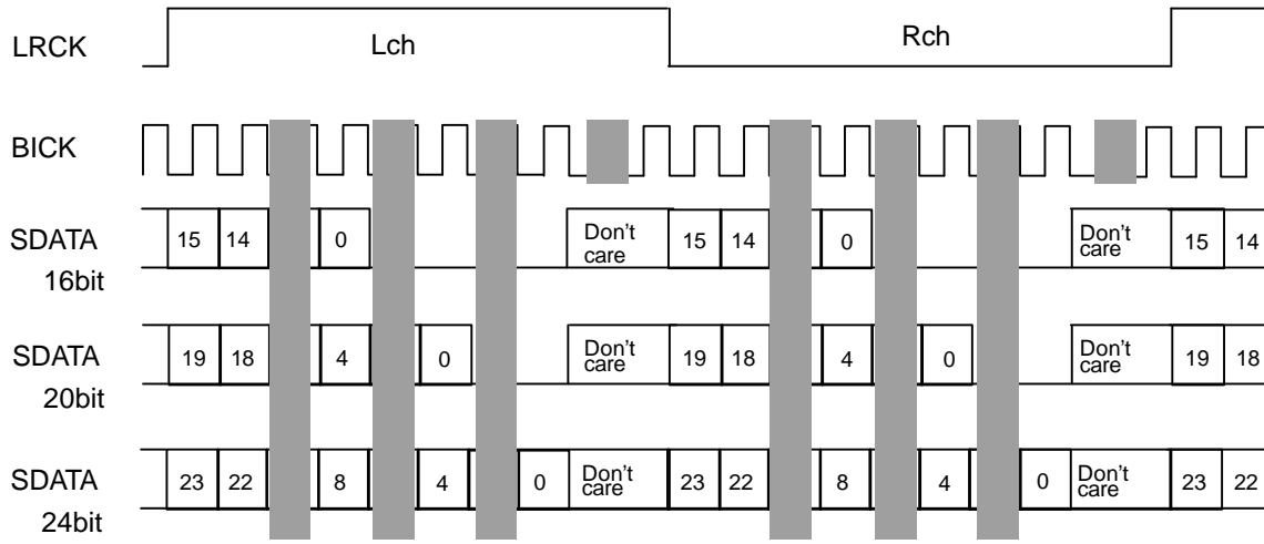
Figure 11. Mode 2 Timing
