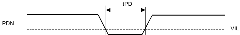
Figure 8. Power-down & Reset Timing
