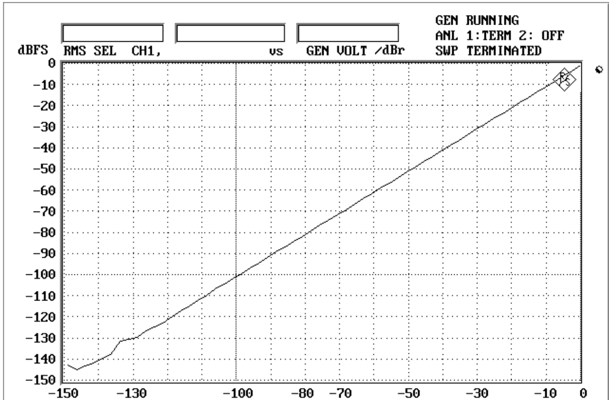
Fig.7 Linearity
