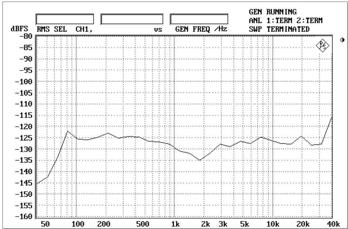
Fig.18 Crosstalk
