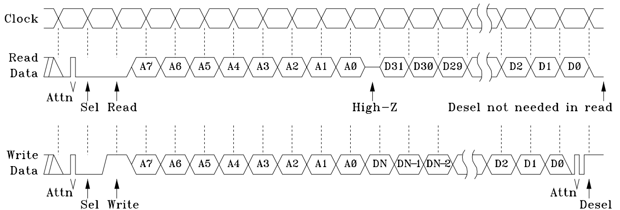
Write Timing
