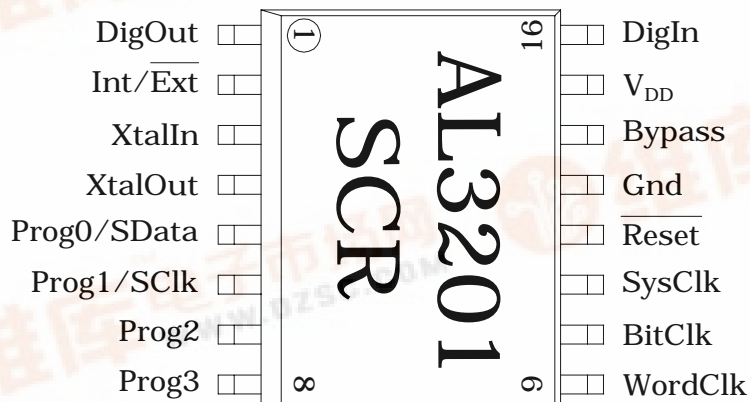
16 pin SOIC 300 mils wide
