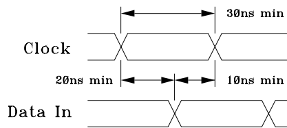
Write Timing
