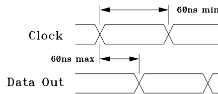
Read Timing
