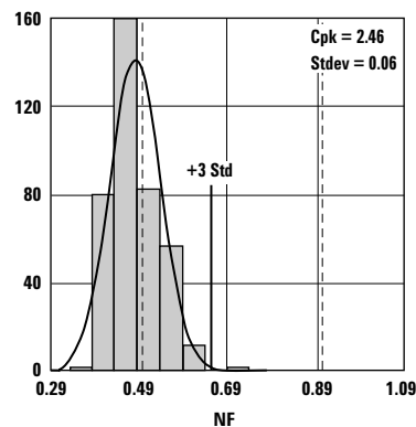
Figure 4. Capability Plot for NF @ 2.7 V, 10 mA. Nominal = 0.5, USL = 0.9
