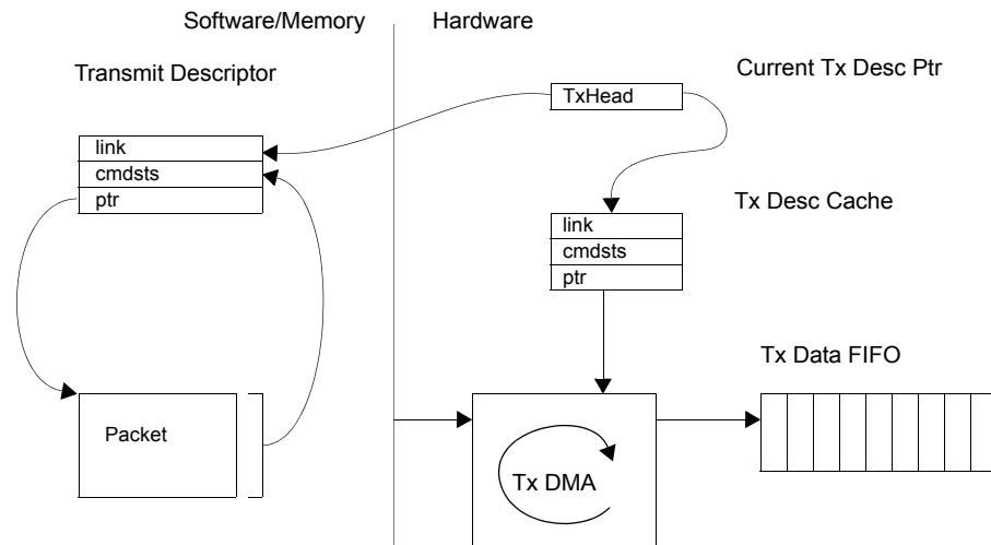
Figure 5-4 Transmit Architecture
