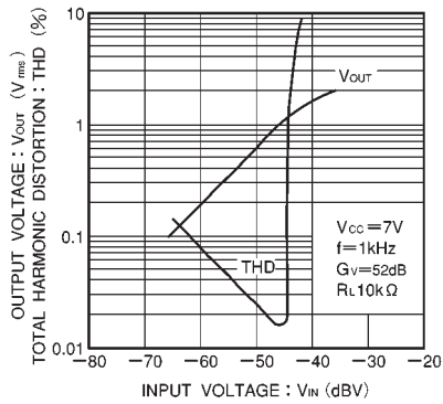
Fig. 18 Input/output characteristics
