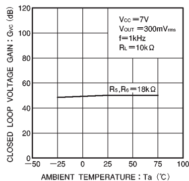
Fig. 14 Closed loop voltage gain vs. ambient temperature
