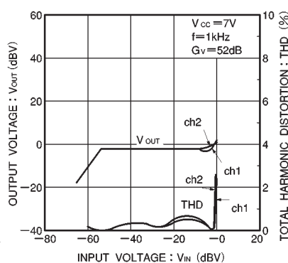
Fig. 17 ALC characteristics
