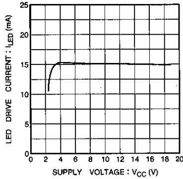
Fig. 3 LED drive current vs. supply voltage
