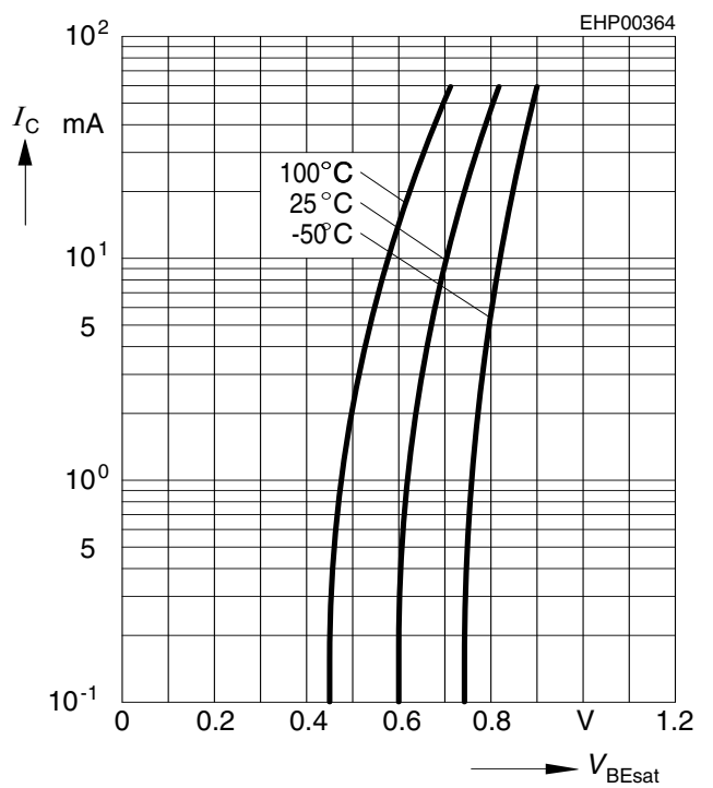
Base-emitter saturation voltage I_C = f(V_{BEsat}), h_{FE} = 20
