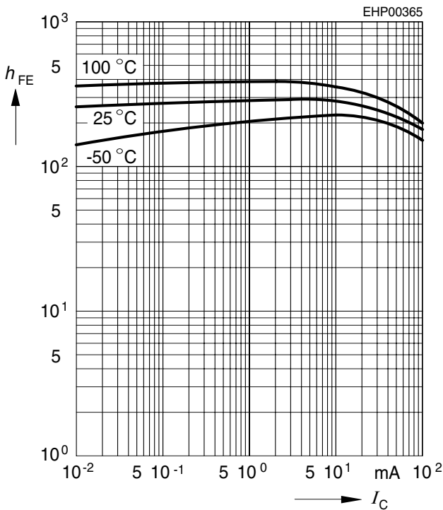
DC current gain h_{FE} = f(I_C) V_{CE} = 5V
