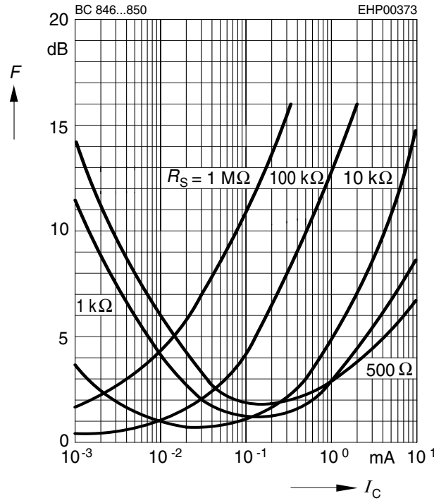
Noise figure F = f(I_C) V_{CE} = 5V, f = 1kHz
