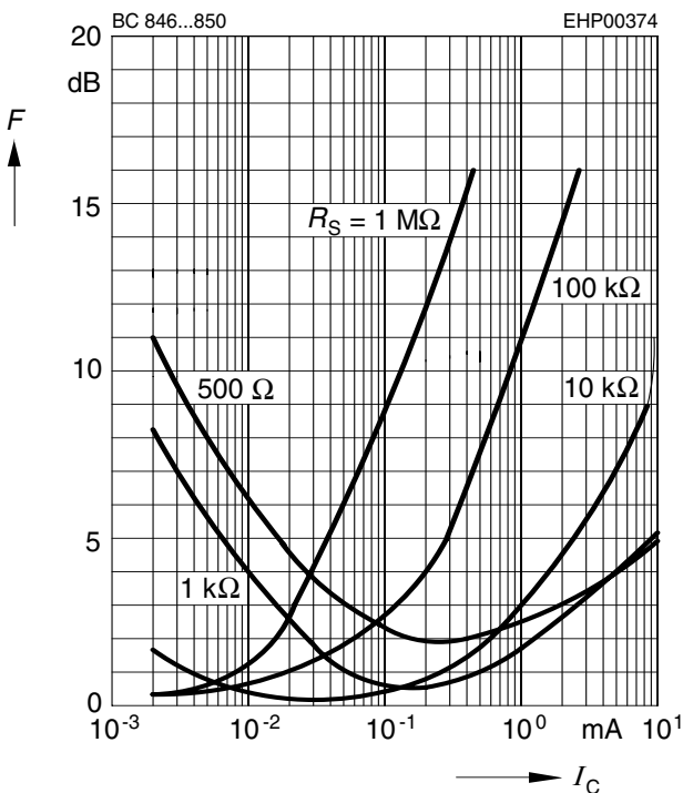
Noise figure F = f(I_C) V_{CE} = 5V, f = 10kHz
