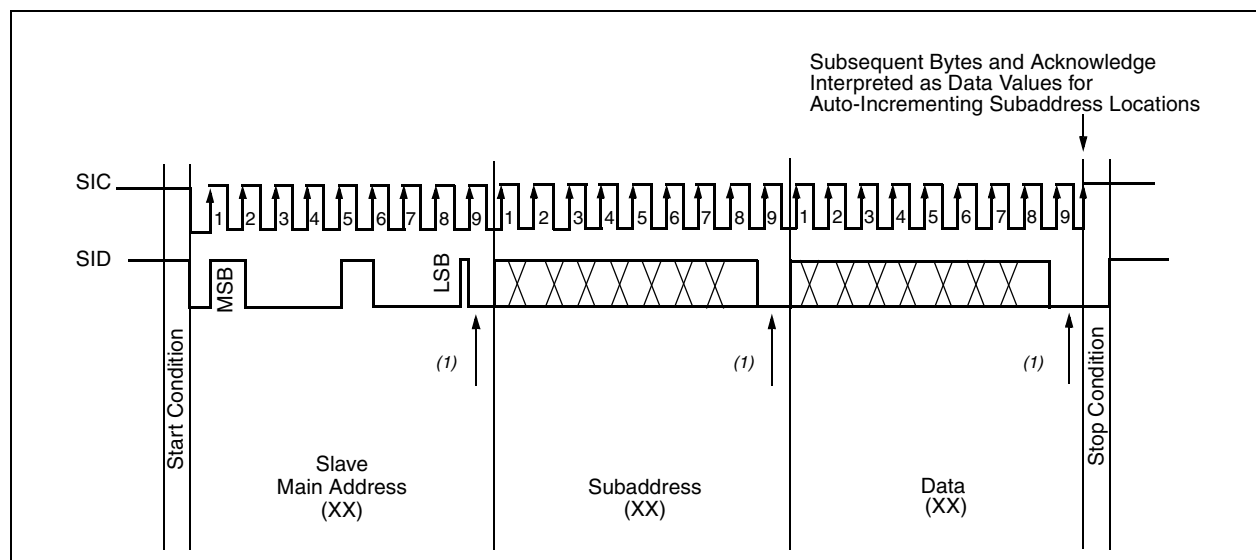
Figure 3-5. SID/SIC Diagram
