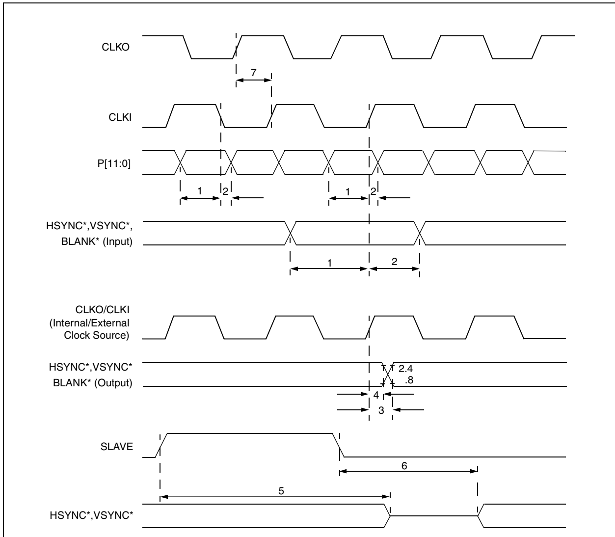
Figure 4-1. Interface Timing
