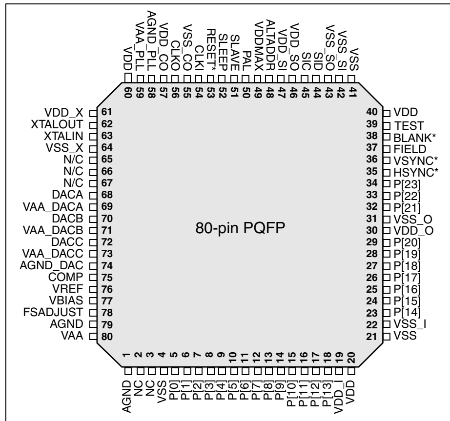
Figure 1-1. Pinout Diagram
