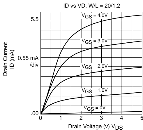
n-ch Transistor IV characteristics of a 20/1.2 device
