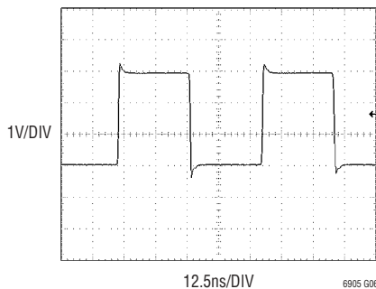
LTC6905 Output Operating at 17.5MHz, V_S = 3V
