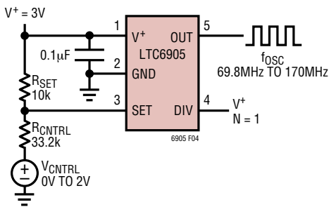
Figure 4. Voltage Controlled Oscillator
