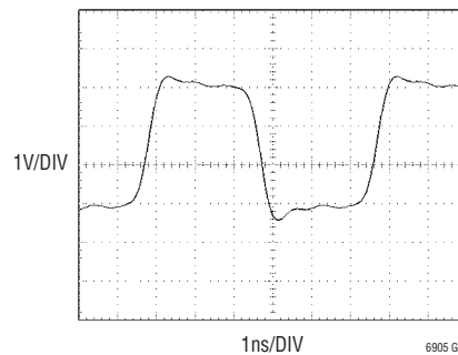
LTC6905 Output Operating at 170MHz, V_S = 3V
