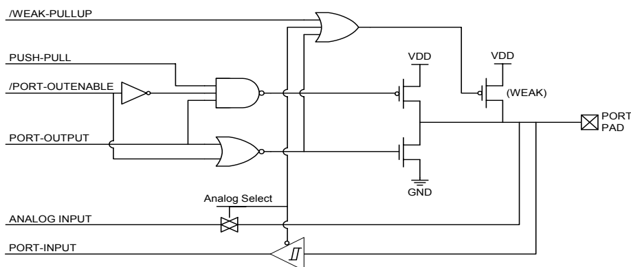
Figure 12.2. Port I/O Cell Block Diagram
