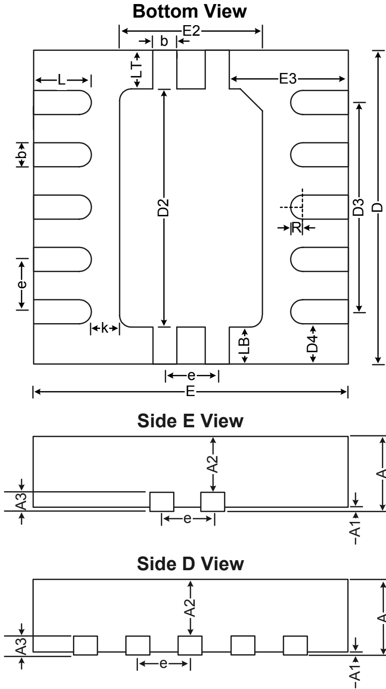
Figure 4.2. QFN-11 Package Drawing
