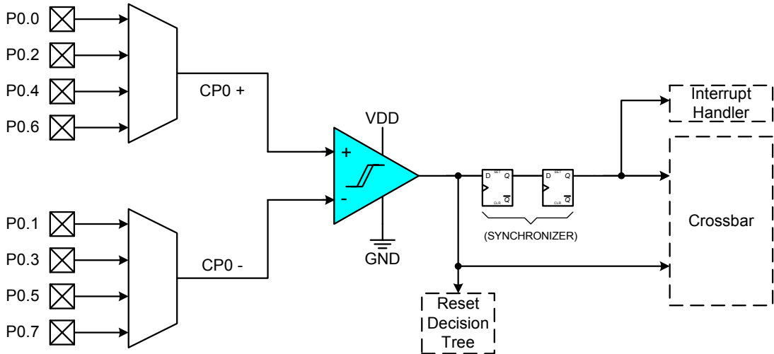
Figure 1.11. Comparator Block Diagram
