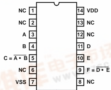
CD40107BF TOP VIEW
