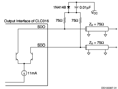
FIGURE 19. Differential Source-Terminated Output Interface
