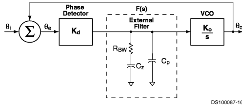
FIGURE 4. PLL Loop
