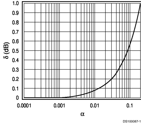
FIGURE 6. Jitter Peaking Curve
