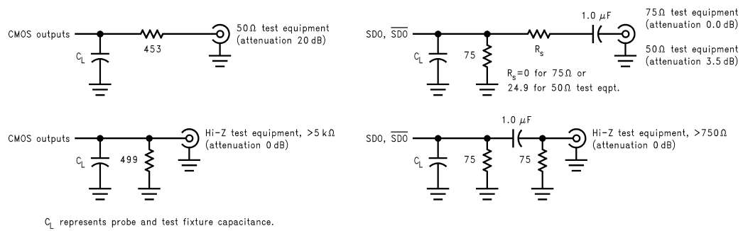
FIGURE 1. Test Loads
