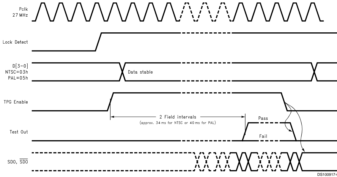
FIGURE 4. Built-In Self-Test Control Sequence
