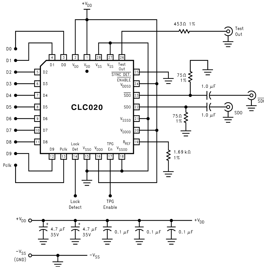
FIGURE 2. Test Circuit
