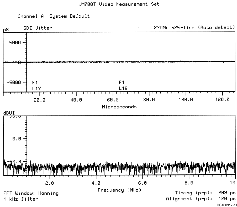
FIGURE 10. Jitter Plots
