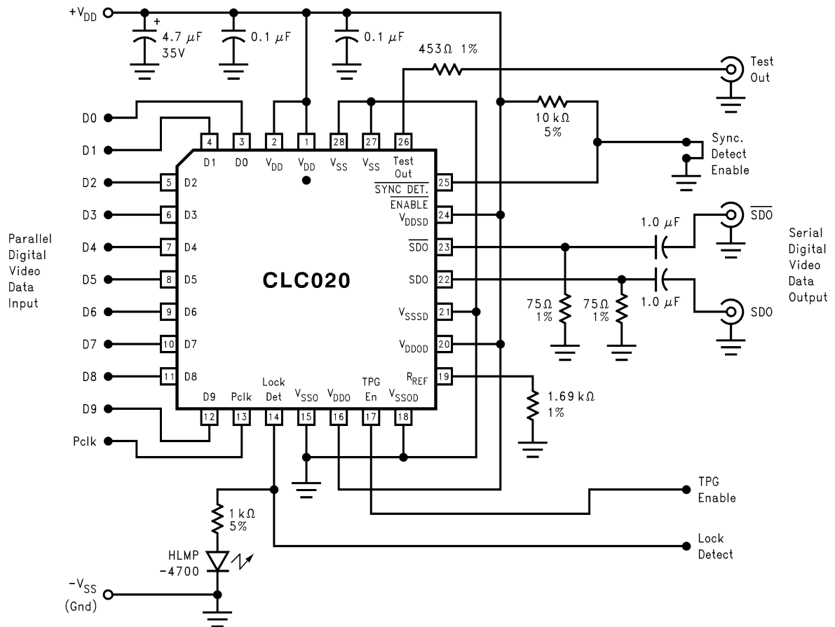
FIGURE 6. Typical Application Circuit
