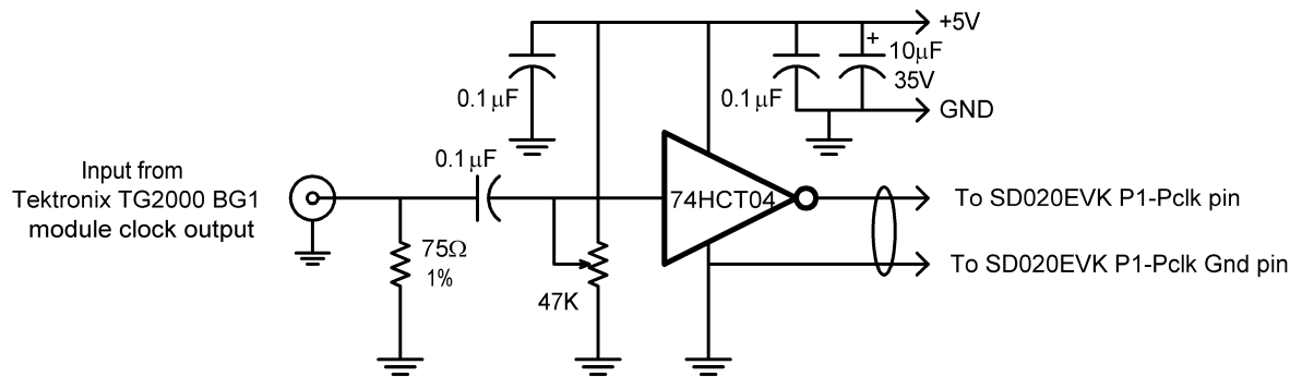
FIGURE 8. Jitter Test Circuit
