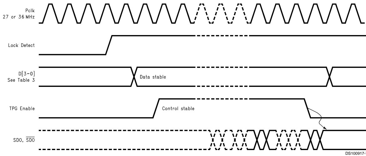
FIGURE 5. Test Pattern Generator Control Sequence
