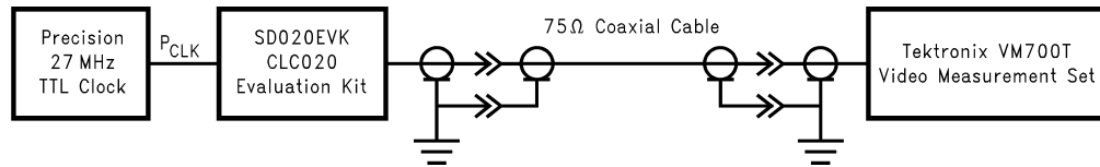
FIGURE 8. Jitter Test Circuit
