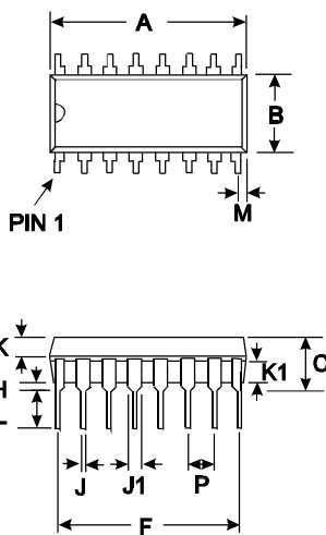
Figure 9 16-pin SOIC (D4) Mechanical Outline: Order as part no. CMX615D4
