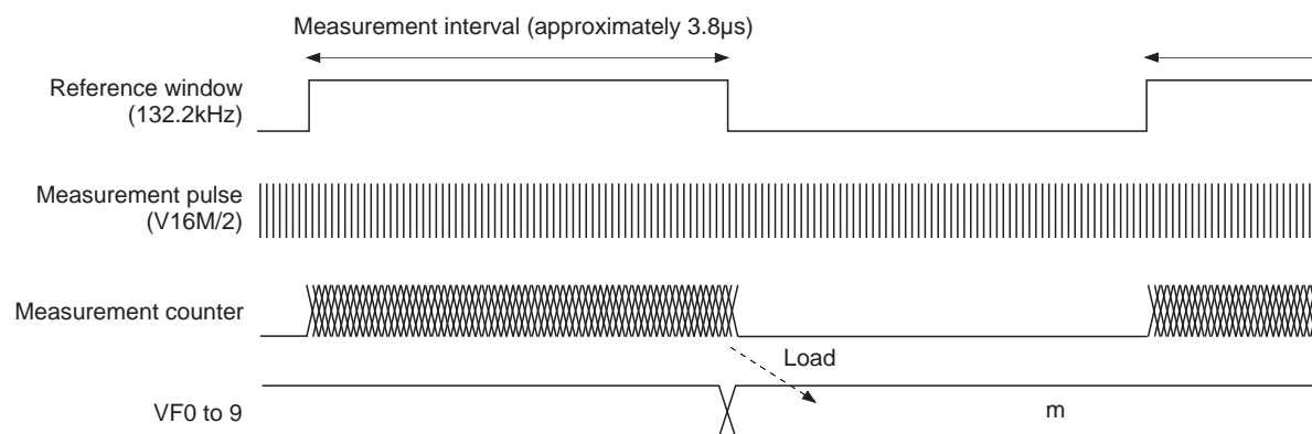
Timing Chart 2-5
