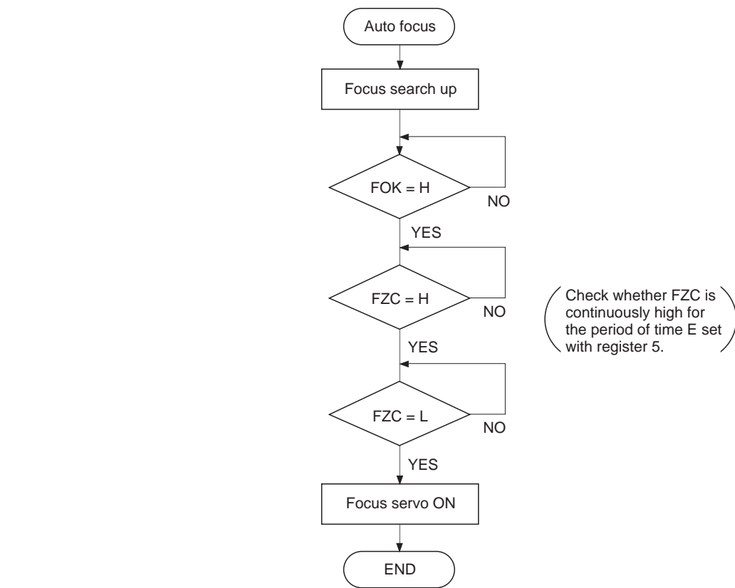
Fig. 4-6-(a). Auto Focus Flow Chart
