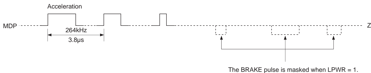
Timing Chart 1-15
