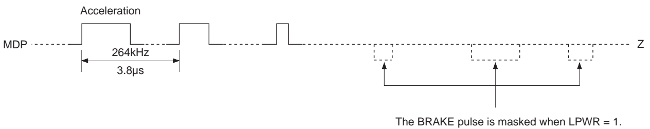
Timing Chart 1-14
