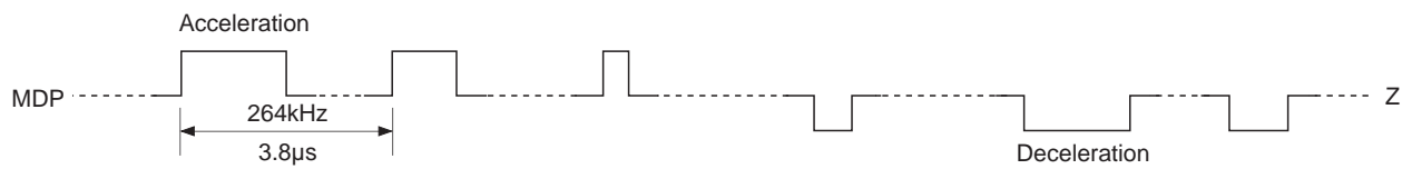
Timing Chart 1-12
