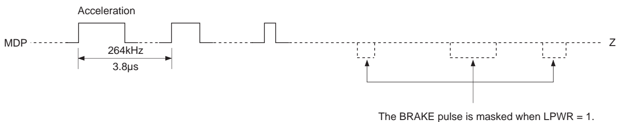
Timing Chart 1-15
