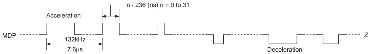
Timing Chart 1-12
