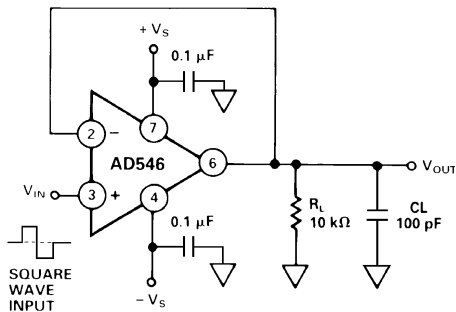
Figure 18. Unity Gain Follower
