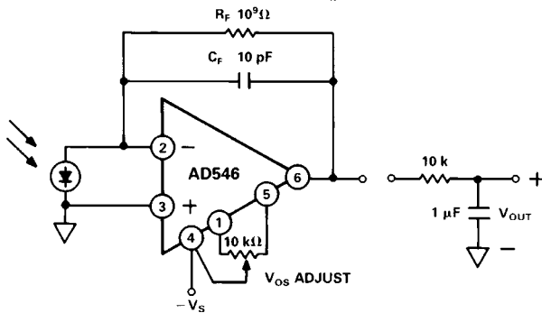
Figure 39. Photodiode Preamp
