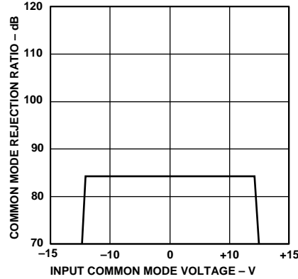
Figure 5. CMRR vs. Input Common-Mode Voltage
