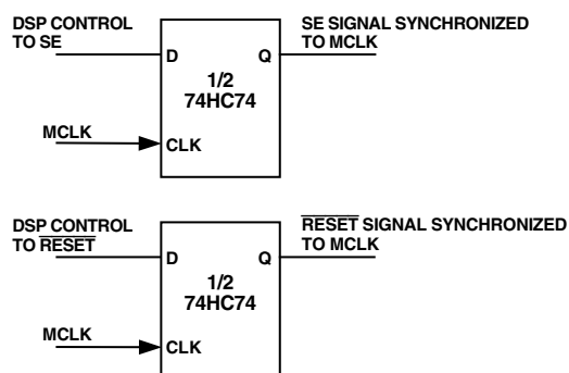
Figure 30. SE and \overline{\text{RESET}} Sync Circuit for Cascaded Operation
