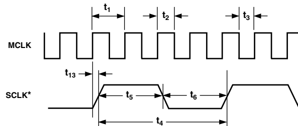
Figure 3. SCLK Timing
