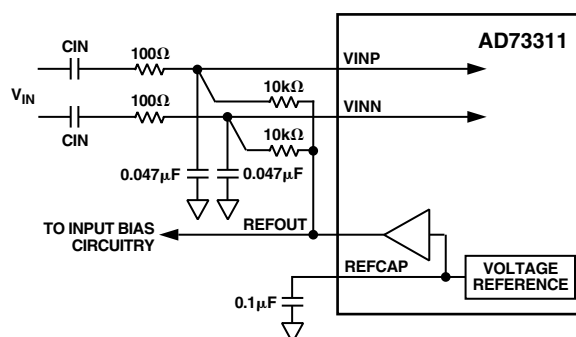
Figure 23. Example Circuit for Differential Input (AC Coupling)
