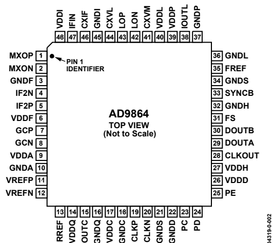
Figure 2. 48-Lead LFCSP, Backside Paddle Contact Is Connected to Ground
