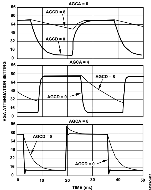
Figure 61. AGC Response for Different AGCA and AGCD Settings with f_{\text{CLK}} = 18 \text{ MSPS} , f_{\text{CLKOUT}} = 20 \text{ KSPS} , Decimate by 900, and AGCO = 0
