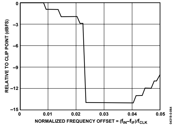
Figure 63. Maximum Interferer (or Blocker) Input Level vs. Normalized IF Frequency Offset
