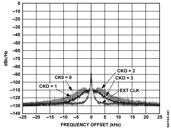
Figure 41. CLK Phase Noise vs. I_{BIAS} Setting ( CKO ) (IF = 73.35 MHz, IF = 71.1 MHz, IFIN = -31 dBm, f_{CLK} = 18 MHz, f_{REF} = 16.8 MHz) (CLK SYN Settings: CKI = 7, CLR = 56, and CLN = 60 with f_{REF} = 300 kHz)
