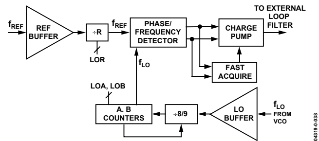
Figure 38. LO Synthesizer
