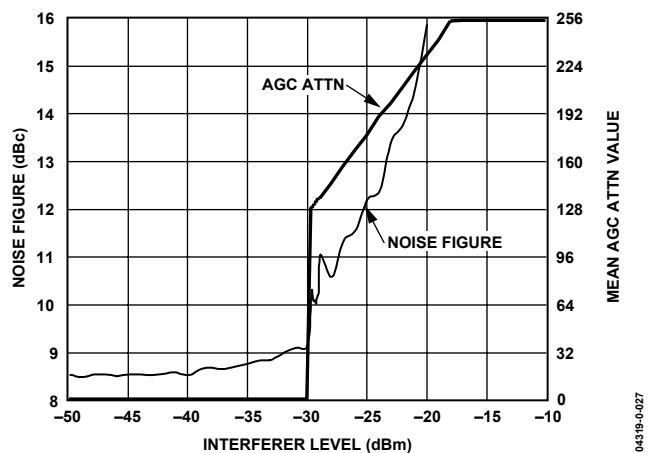
Figure 27. Noise Figure vs. Interferer Level (16-Bit Data with DVGA, BW = 12.5 kHz, AGCR = 1 , f_{\text{INTERFERER}} = f_{\text{IF}} + 110 kHz)
