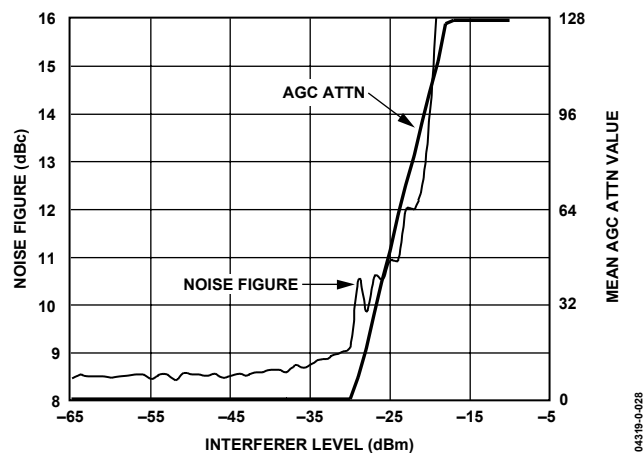
Figure 28. Noise Figure vs. Interferer Level (24-Bit Data, BW = 12.5 kHz, AGCR = 1 , f_{\text{INTERFERER}} = f_{\text{IF}} + 110 kHz)
