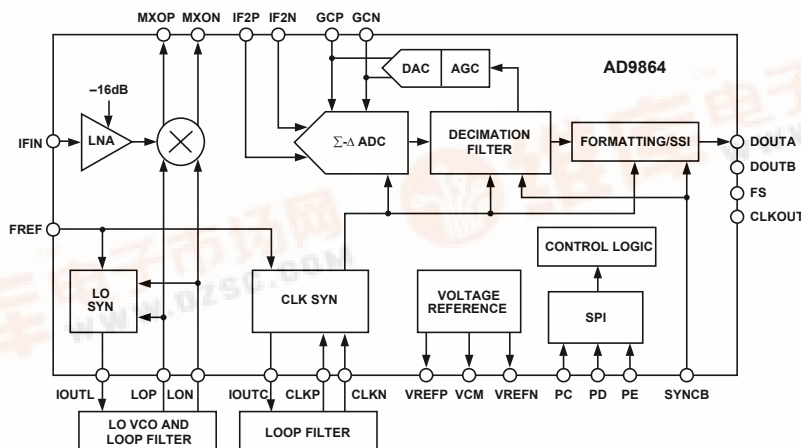
Figure 1. AD9864 Block Diagram
