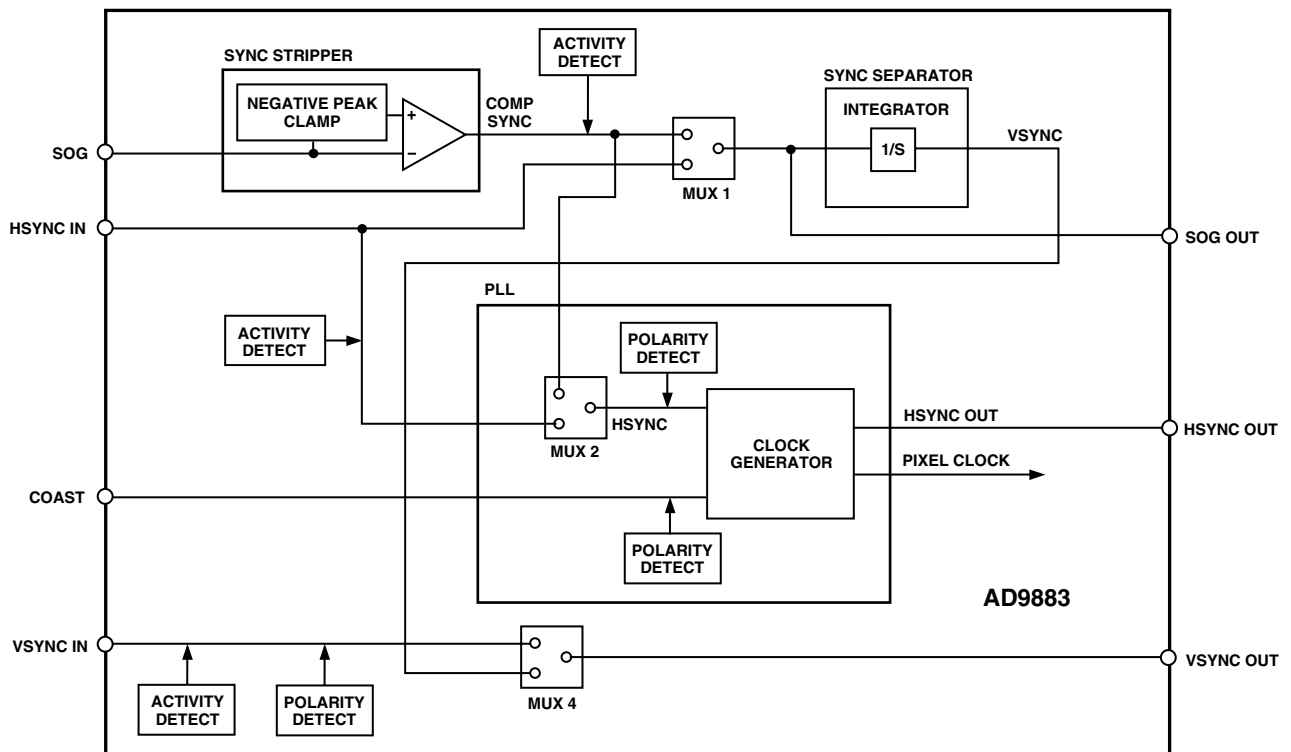
Figure 11. Sync Processing Block Diagram
