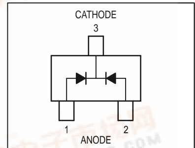
CASE 463-01, STYLE 4 SOT-416/SC-90
