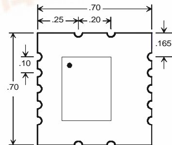
DR4001 Outline Drawing
