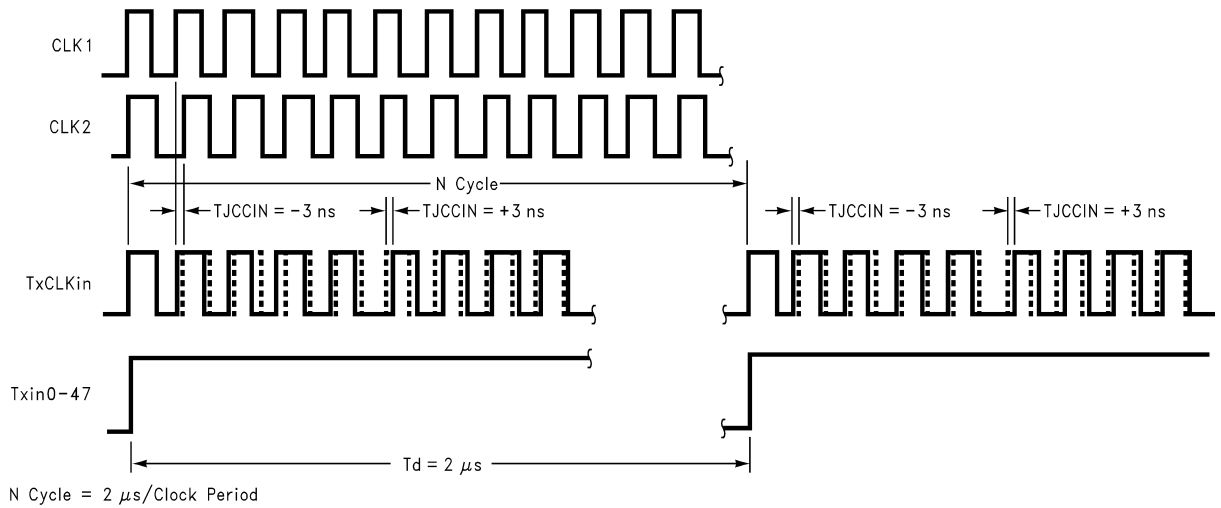
FIGURE 15. Timing Diagram of the Input Cycle-to-Cycle Clock Jitter
