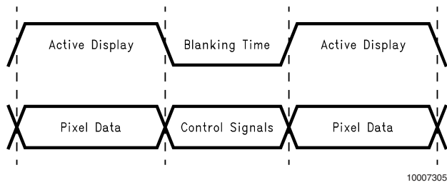
FIGURE 19. Control Signals Transmitted During Blanking
