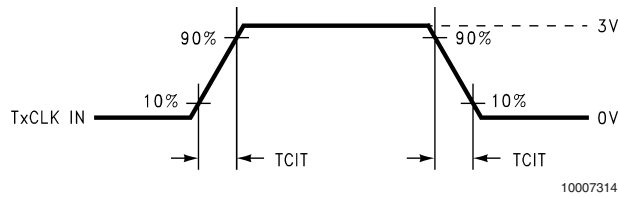
FIGURE 5. DS90C387 (Transmitter) Input Clock Transition Time
