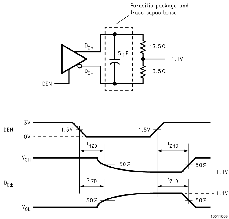
FIGURE 7. Serializer TRI-STATE Test Circuit and Timing
