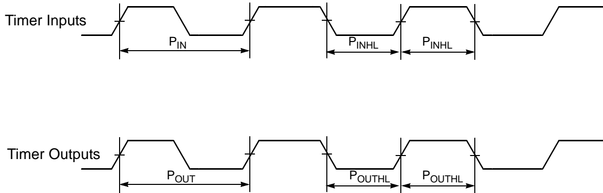
Figure 23. Timer Timing
