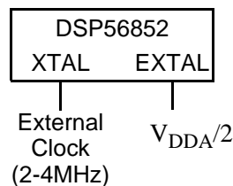
Figure 10. Connecting a Low Speed External Clock Signal using XTAL
