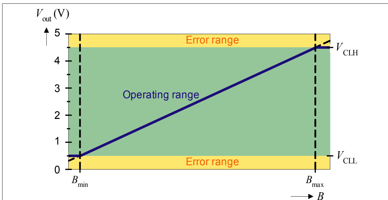
Figure 5 Clamping
