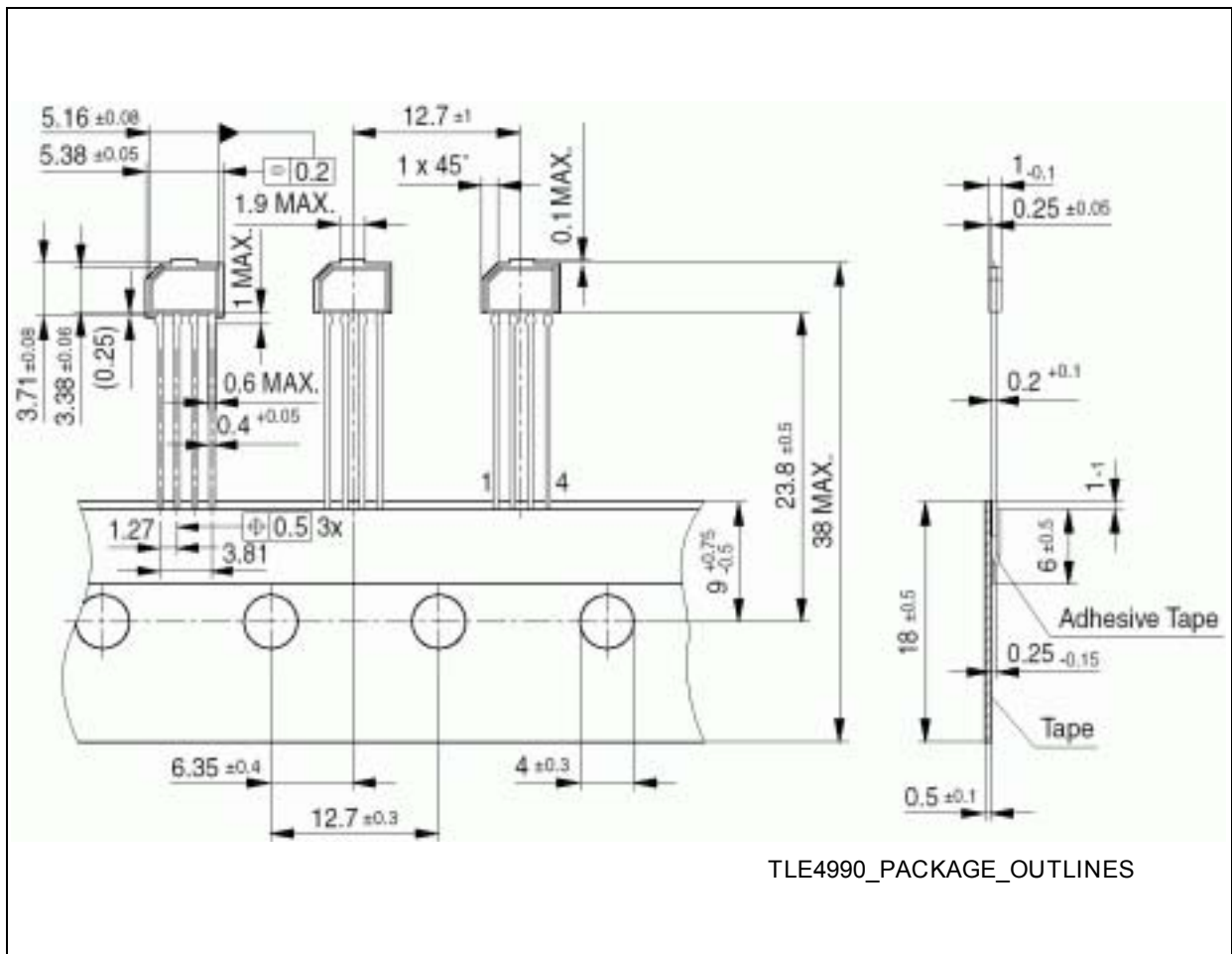
Figure 7 Package Outline
