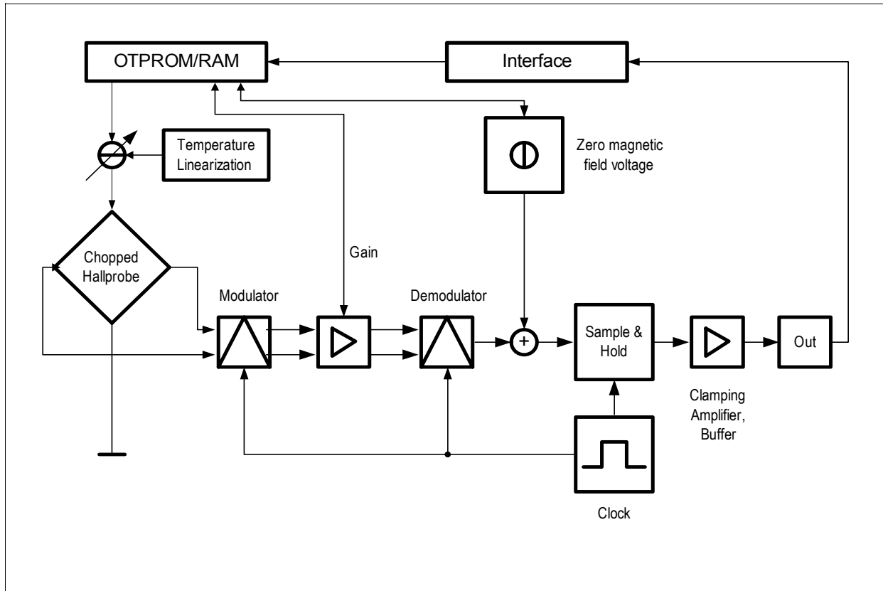
Figure 2 Block Diagram
