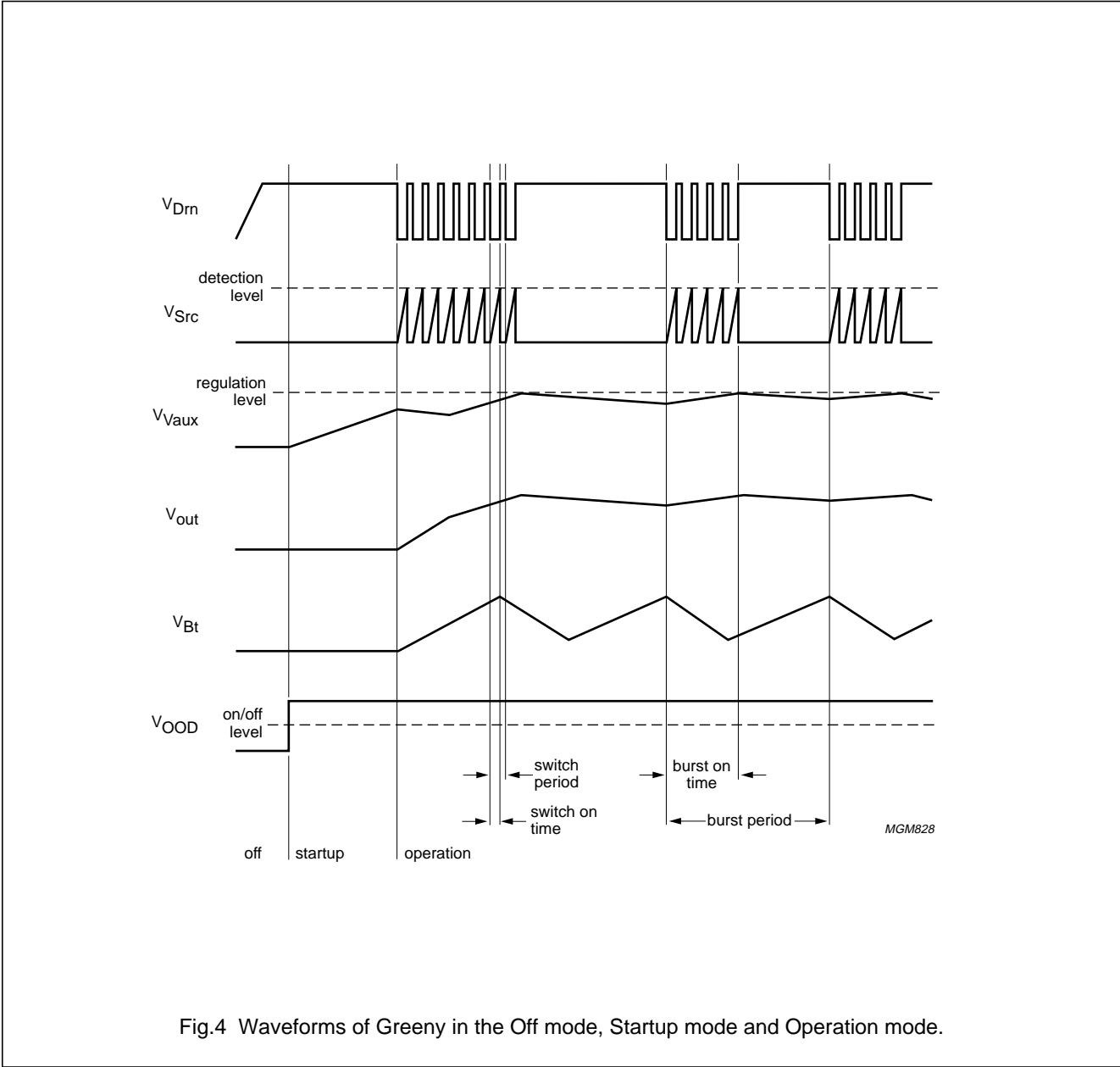
Waveforms of Greeny in the Off mode, Startup mode and Operation mode
