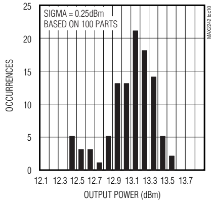
OUTPUT POWER HISTOGRAM AT FIXED 0.8V POWER DETECTOR VOLTAGE
