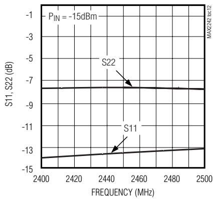
S11, S22, vs. FREQUENCY
