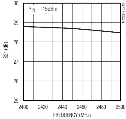
MAX2242 S21 vs. FREQUENCY
