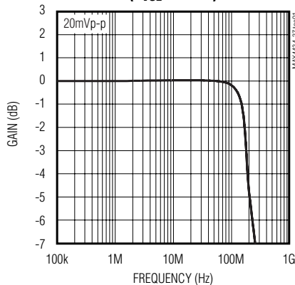
MAX4434/MAX4436 SMALL-SIGNAL GAIN vs. FREQUENCY ( A_{VCL} = +1V/V )
