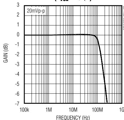
MAX4435/MAX4437 SMALL-SIGNAL GAIN vs. FREQUENCY ( A_{VCL} = +5V/V )
