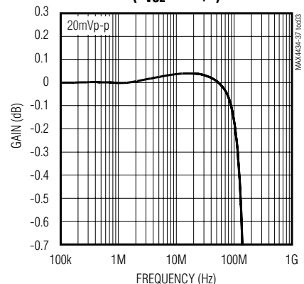
MAX4434/MAX4436 GAIN FLATNESS vs. FREQUENCY ( A_{VCL} = +1V/V )
