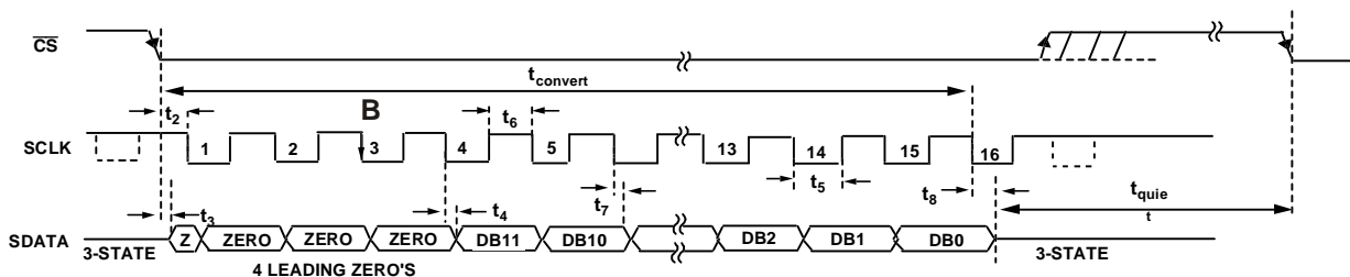
Figure 15. AD7466 Serial Interface Timing Diagram
