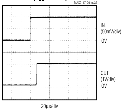
MAX9117/MAX9119 PROPAGATION DELAY ( t_{PD+} ) ( V_{CC} = +1.8V )
