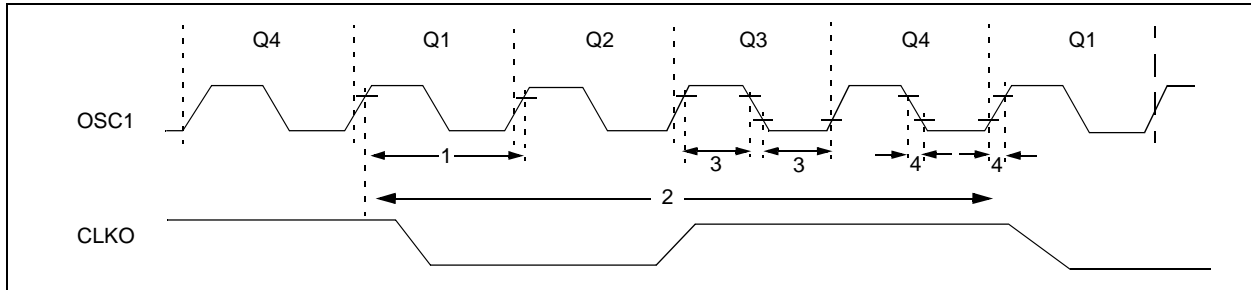
FIGURE 27-5: EXTERNAL CLOCK TIMING (ALL MODES EXCEPT PLL)
