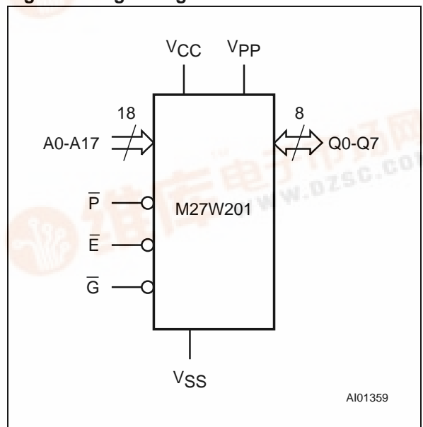
Figure 1. Logic Diagram
