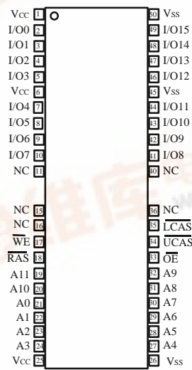
44(50) TSOP II
