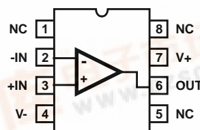
HFA1105 (PDIP, SOIC) TOP VIEW
